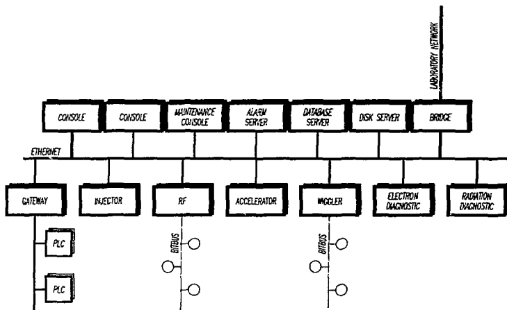
Fig. 2 - The hardware architecture of the control system
