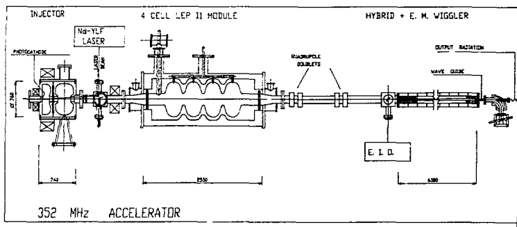
Fig.1 -General layout of the ELFA experiment
