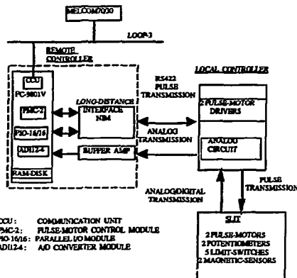
Fig. 3 Block Diagram of the Slit Control System
