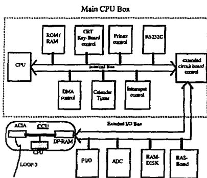
Fig. 4 Configuration of FC-9801V
