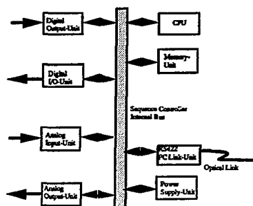
Fig. 6 Sequencer System
