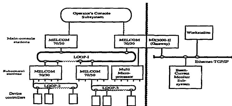
Fig. 1 Block Diagram of the PF Linac Control System
