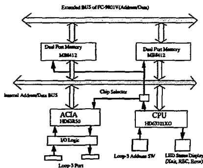
Fig. 5 Configuration of the CCU
