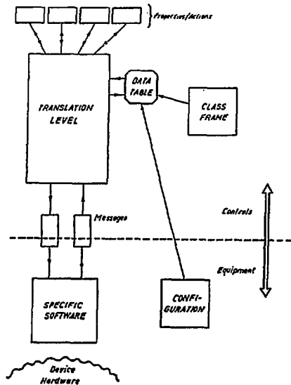
Figure 2. A general implementation scheme
