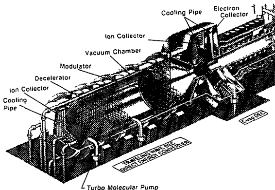
Fig.5 The schematic drawing of the proposed DEC's , i.e., the cusp-type DEC and the traveling wave DEC
