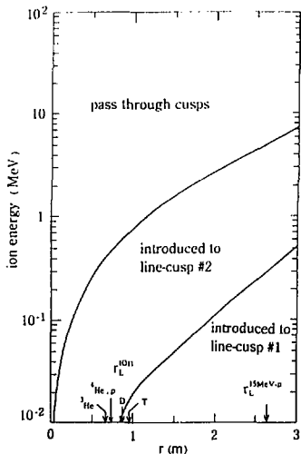
Fig.2 The particle classification diagram in ion energy and incident radius space, here as reference the characteristic radii of ions are also indicated.
