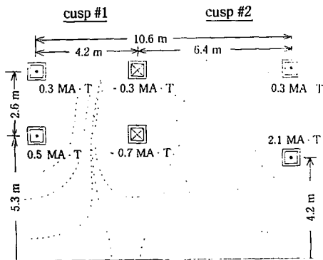
Fig.1 The arrangement of cusp type DEC : the radii, distances and currents of cusp coils : The incident particles come from the left side. The magnetic field lines are also shown by dashed lines.
