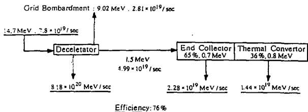
Fig. 4 The energy flow diagram of traveling wave DEC. The conversion efficiency of the traveling wave DEC is estimated as high as 0.76
