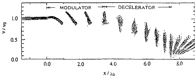
Fig.3 The phase trajectory of fusion protons in the traveling wave DEC.
