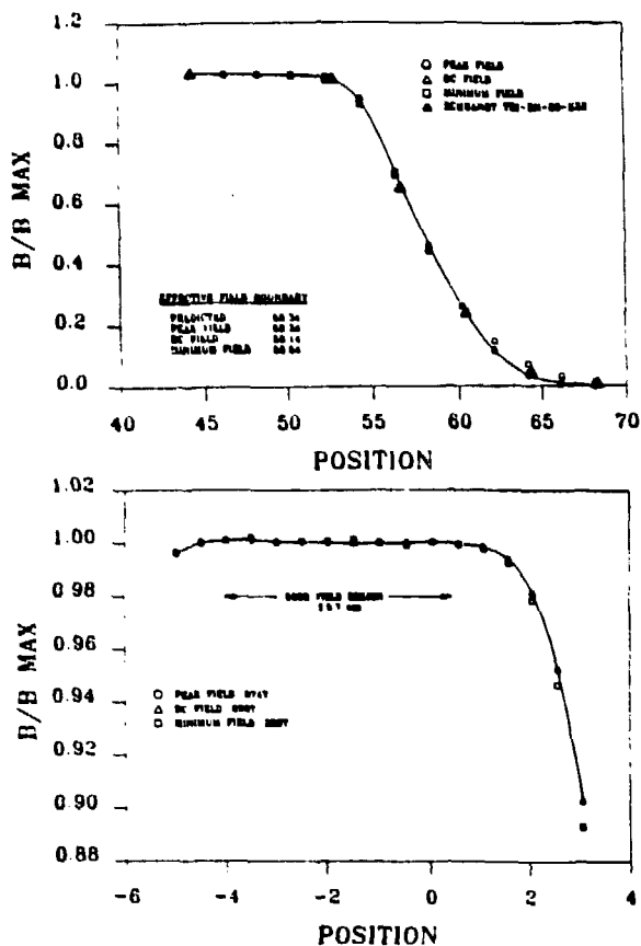
Figure 3 a) Effective length and b) transverse field profile measured at 3000 A dc and 860 A rms ac @ 50 Hz.
