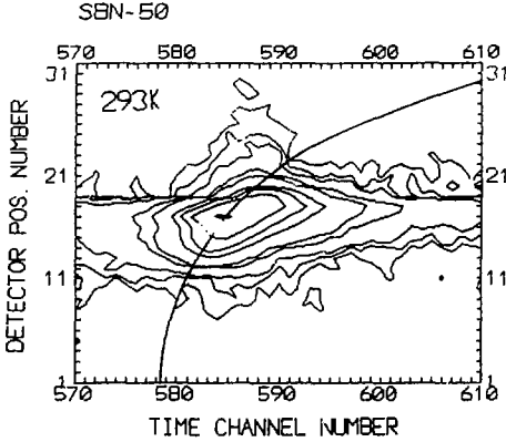
Figure 7: Plot of (001) reflection of SBN-50 around 2\theta = 90^\circ . Diffuse scattering mainly due to other processes than TDS. ( 2\theta -range 78.5^\circ - 101.5^\circ ; ch_w = 64 \mu s )
