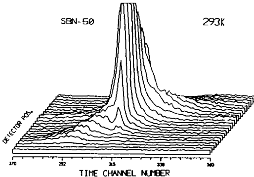
Figure 4: 3d-plot of (002) reflection of SBN-50 around 2\theta = 92.4^\circ . ( 2\theta -range 86.3^\circ - 98.5^\circ , ch_w = 64 \mu s )
