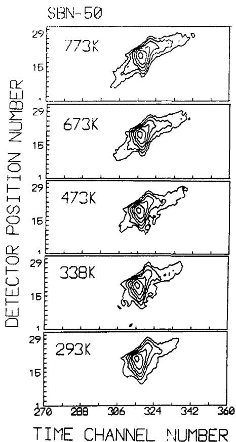
Figure 8: Plot of (002) reflections of SBN-50 around 2\theta = 90^\circ at RT and above (773, 673, 473, and 338 K). ( 2\theta -range 78.5^\circ - 101.5^\circ ; ch_w = 64 \mu s )
