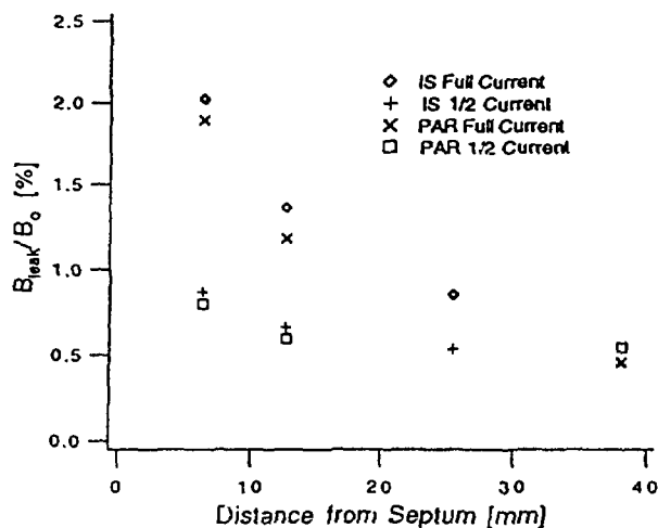
Figure 4: Eddy-current magnet with 0.7 mm steel face shield. Measurements at two different currents.
