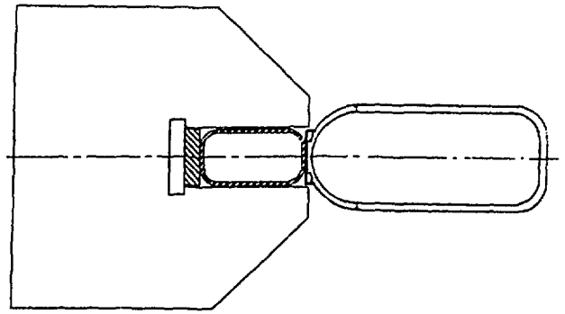
Figure 5: Direct-driven Septum Magnet Cross Section
