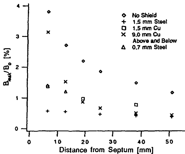
Figure 2: Measurement of the Eddy-current Magnet
