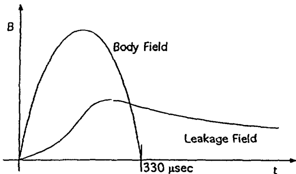
Figure 3: Generic Time Structure of Fields (different vertical scales used for clarity)
