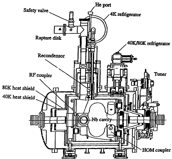
Fig.1.The JAERI superconducting accelerator module cryostat
