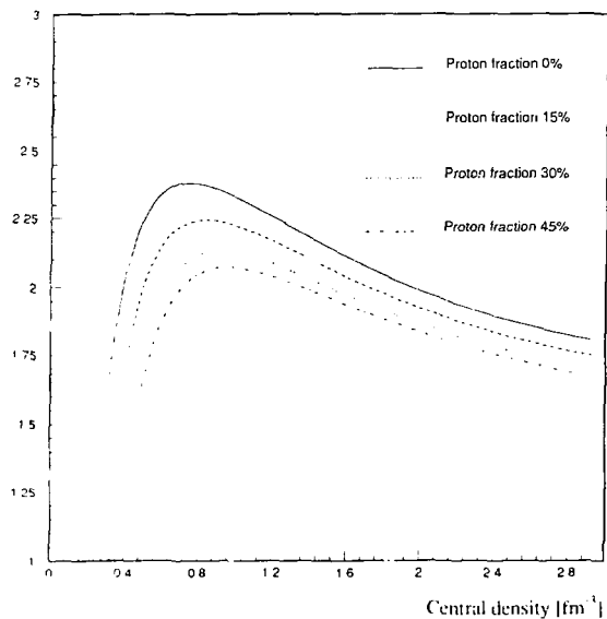
FIG. 2. M_{\max} for various proton fractions as function of the central density \rho_c .
