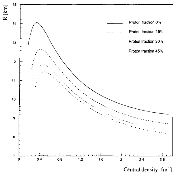
FIG. 3. The total radius R for different proton fractions as function of the central density n_c .
