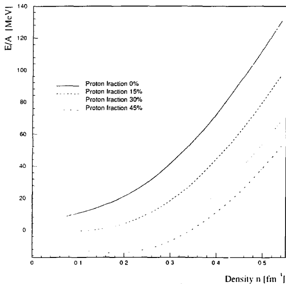
FIG. 1 The energy per particle for asymmetric nuclear matter as function of the particle density for different proton fractions.
