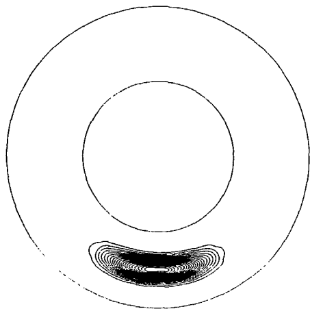
(a) Plasma Stream Line
