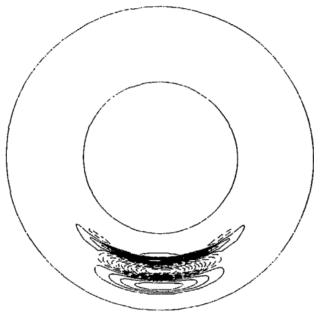
(b) Field-Aligned Current
