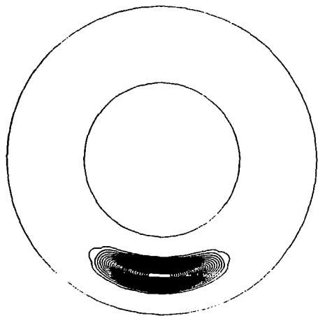
(a) Electrostatic Potential
