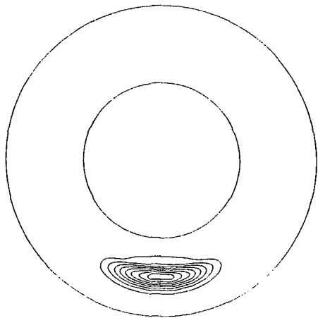
(a) Electrostatic Potential
