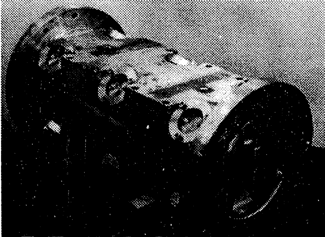
Figure 4: 530 MHz Brazed Engineering Model RFQ
