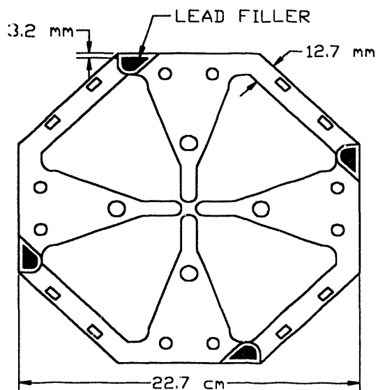
Figure 2: Electroformed 350 MHz RFQ Linac
