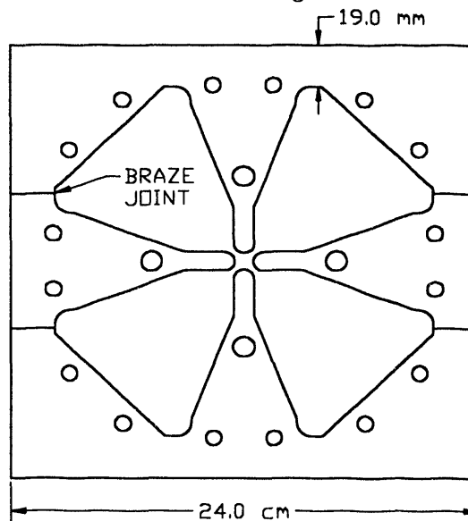
Figure 3: Brazed 350 MHz RFQ Linac
