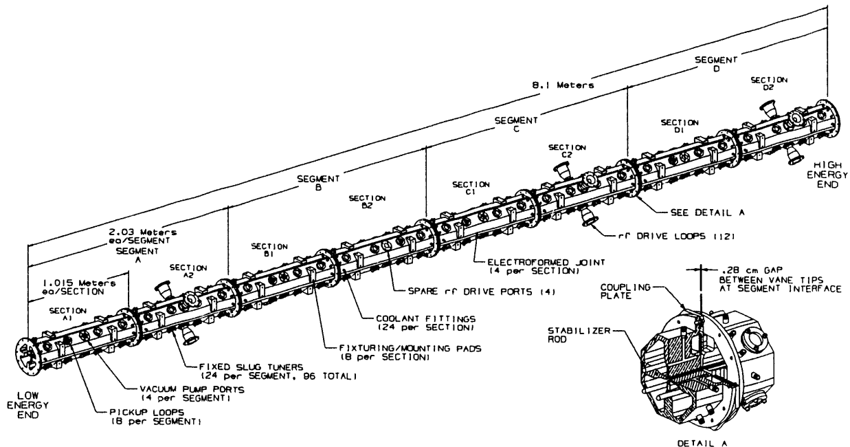
Figure 1: APDF 7 MeV 350 MHz RFQ
