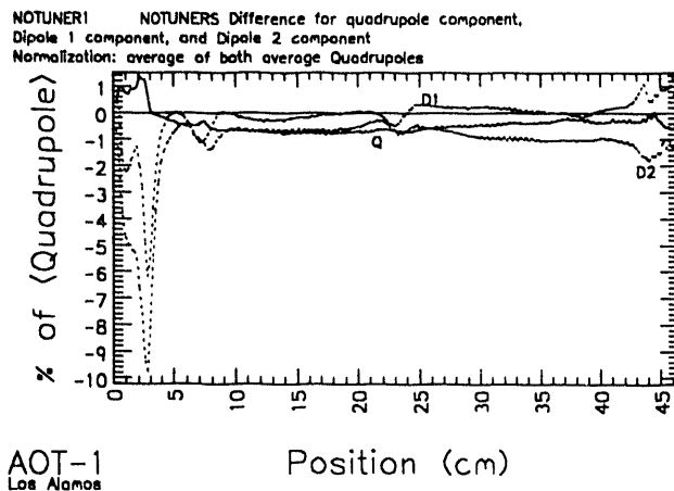
Figure 5: Pre- & Post-Braze Beadpulls
