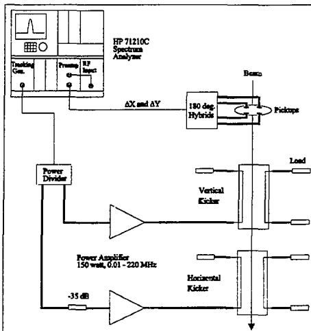
Fig. 2 Block diagram of fractional tune measurement system.
