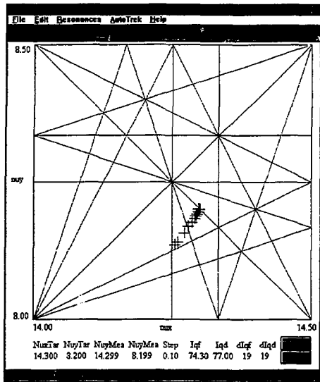
Fig. 3 Tune correction program graphic user interface.
