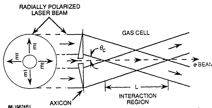
Figure 1: Axicon ICA schematic.
