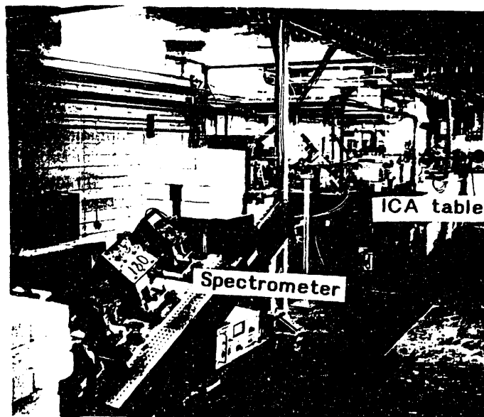
Figure 2: Inverse Cerenkov acceleration beam line.
