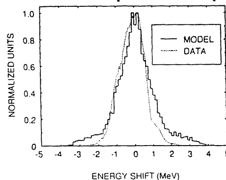
Figure 4: Electron energy spectrum for 0.7 GW laser power.
