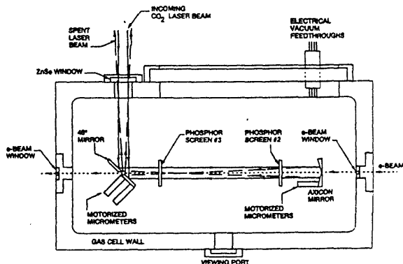
Figure 3: Inverse Cerenkov acceleration gas cell.
