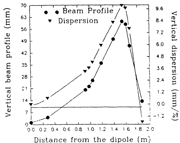
Figure 5: Vertical electron beam profile and dispersion in the spectrometer.
