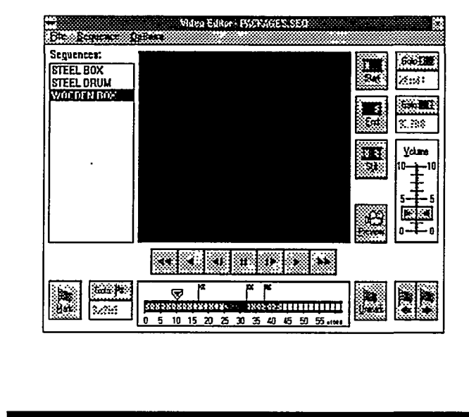
Fig. 2. Video sequencer.
