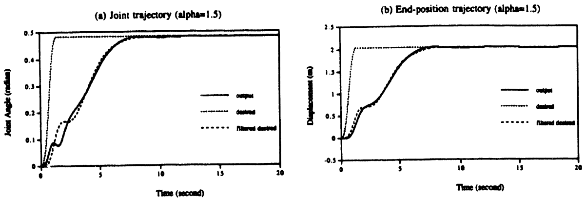
Figure 4. Responses of the robust notch filter with the joint proportional-derivative controller.
