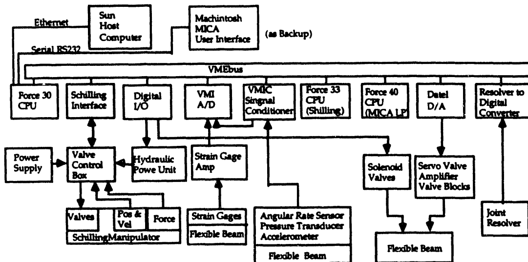
Figure 2. VME system controller for the flexible-beam testbed.
