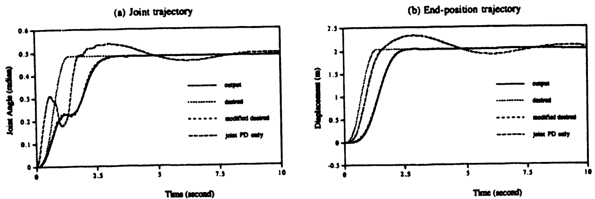
Figure 5. Responses of feedforward simulation filtering method with the joint proportional-derivative controller.
