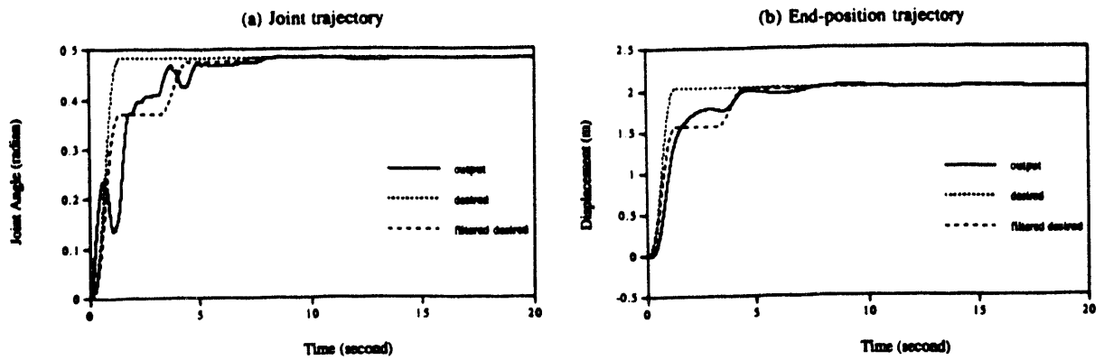
Figure 3. Responses of the impulse shaping filter with the joint proportional-derivative controller.
