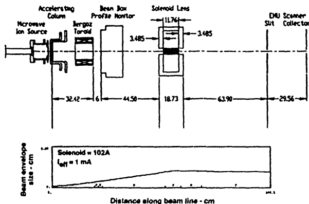
Fig. 1. Schematic layout of the single-solenoid LEBT system for beam transport to the EMU.
