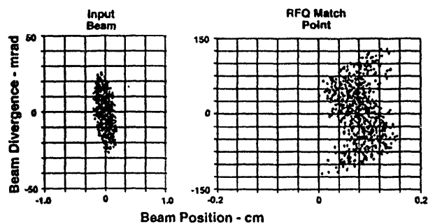
Fig. 4. Calculated phase space distributions in the single-solenoid LEBT.
