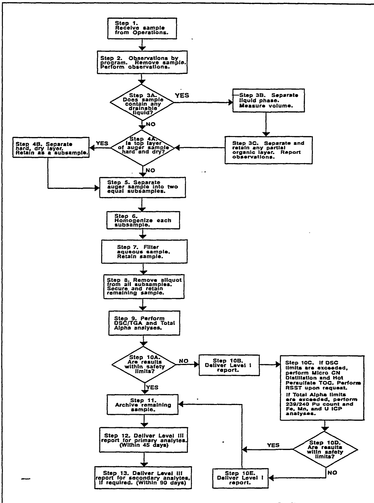
Figure 2: Test Plan Flowchart for Tank Safety Screening.
