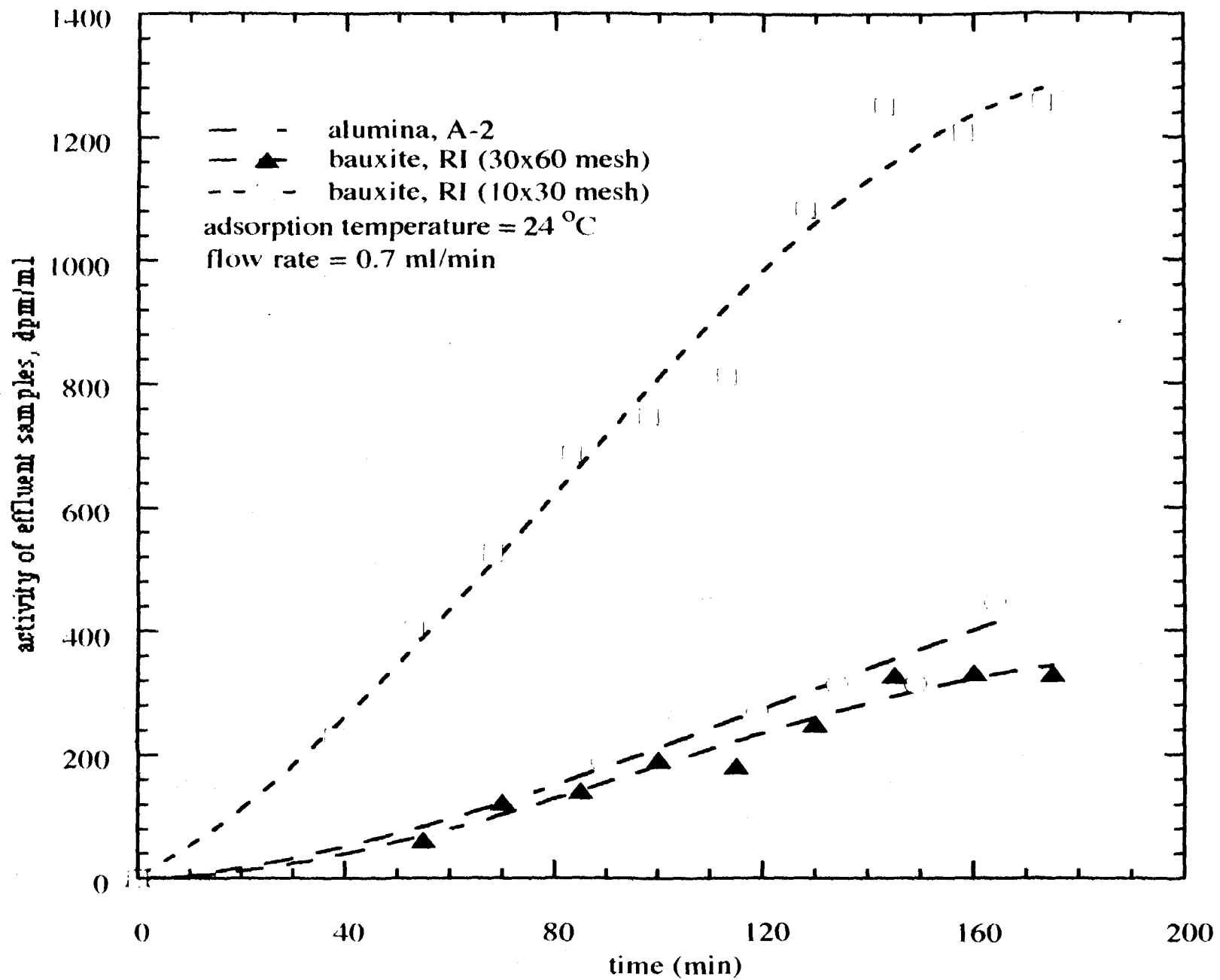
Figure 4. Experimental breakthrough curves of degradation products on adsorbent samples.
