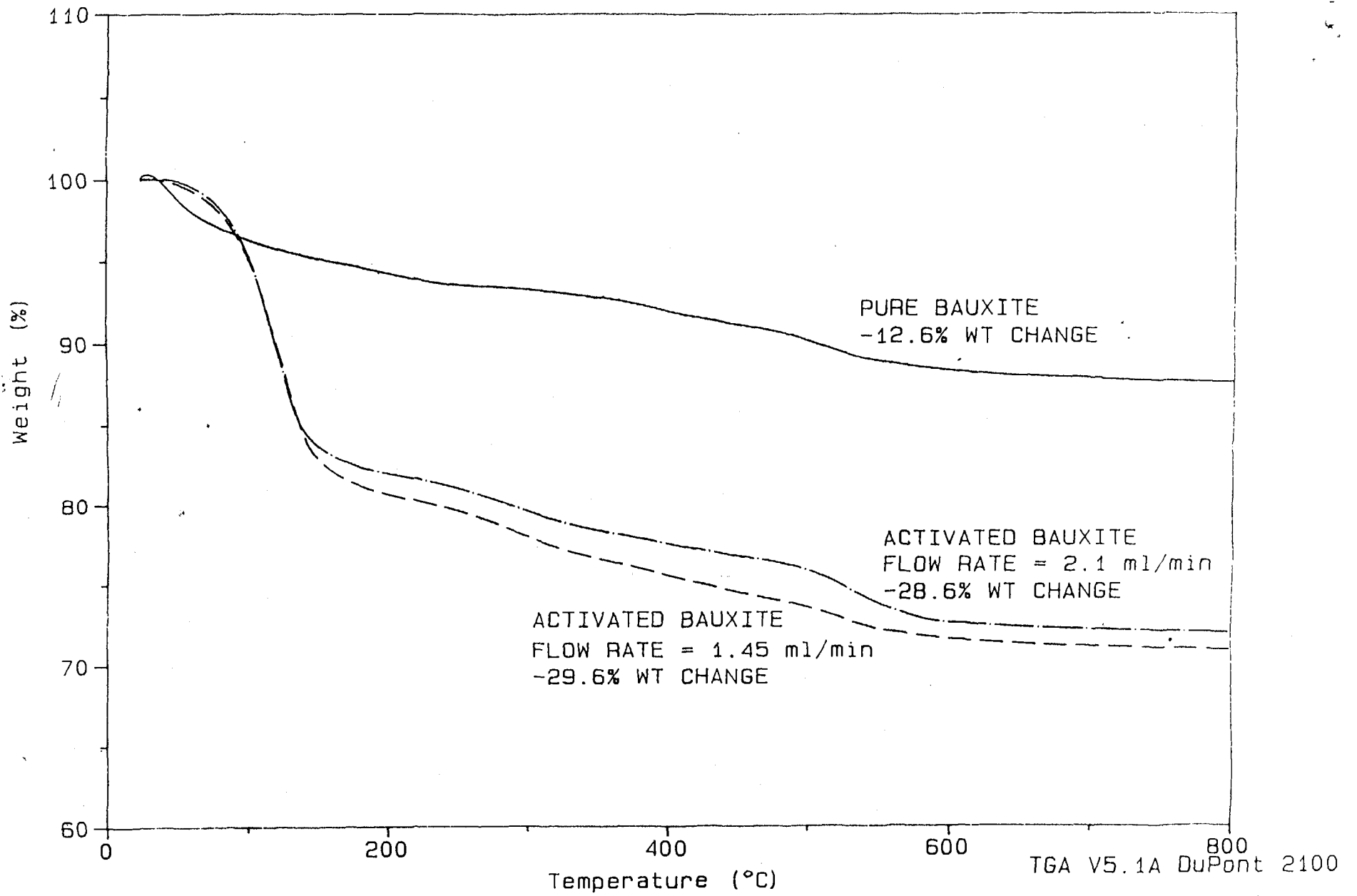
Figure 3. TGA weight loss curves on activated bauxite
