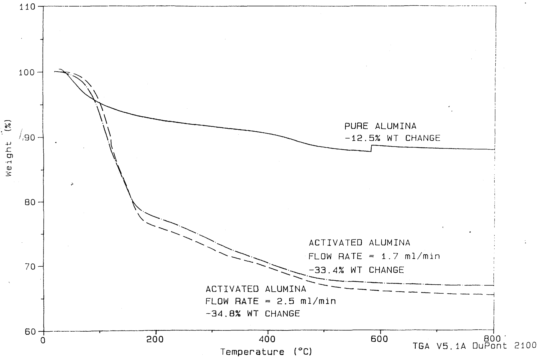
Figure 2. TGA weight loss curves on activated alumina
