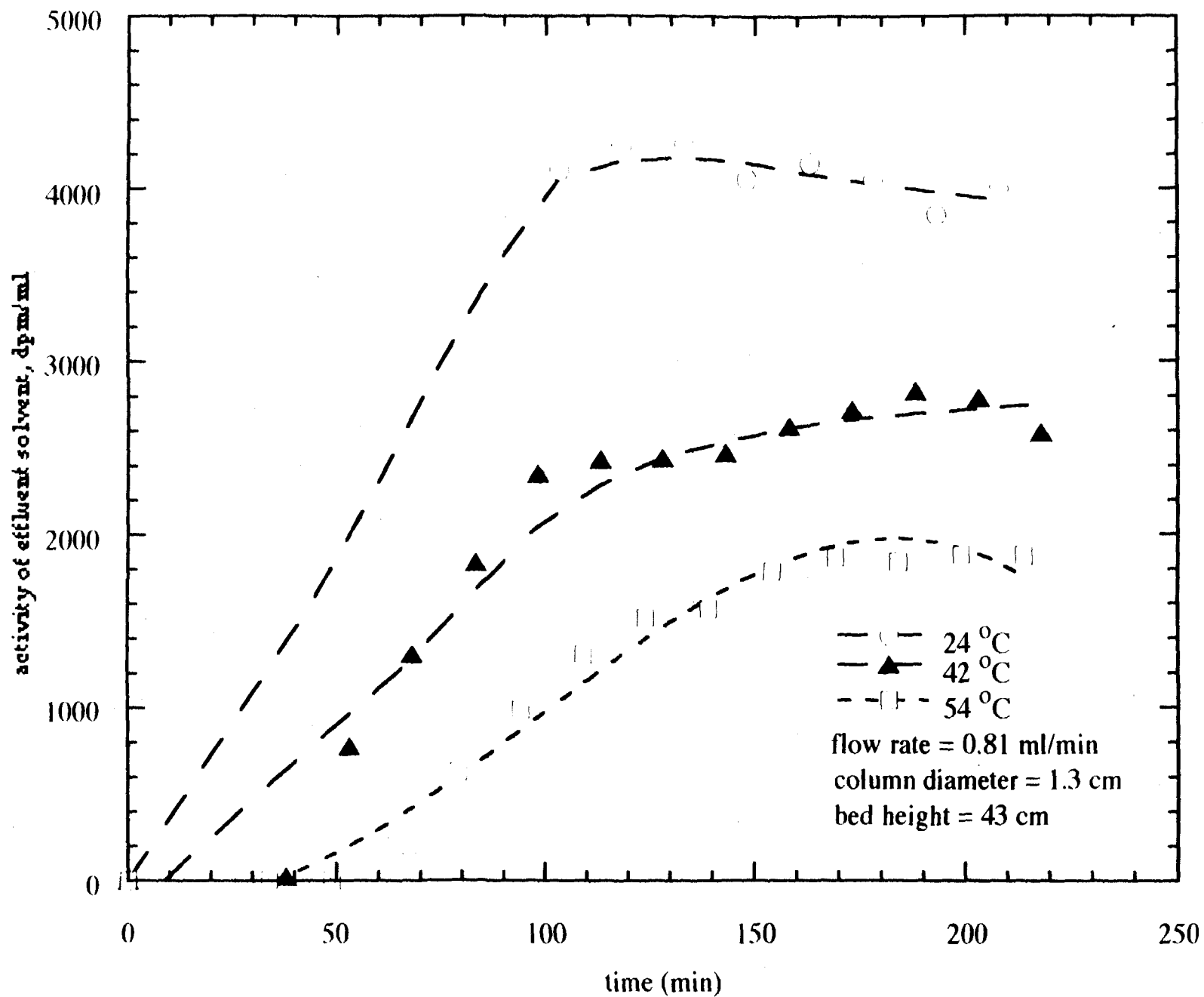
Figure 5. Temperature effects on adsorption of degradation productson activated alumina.
