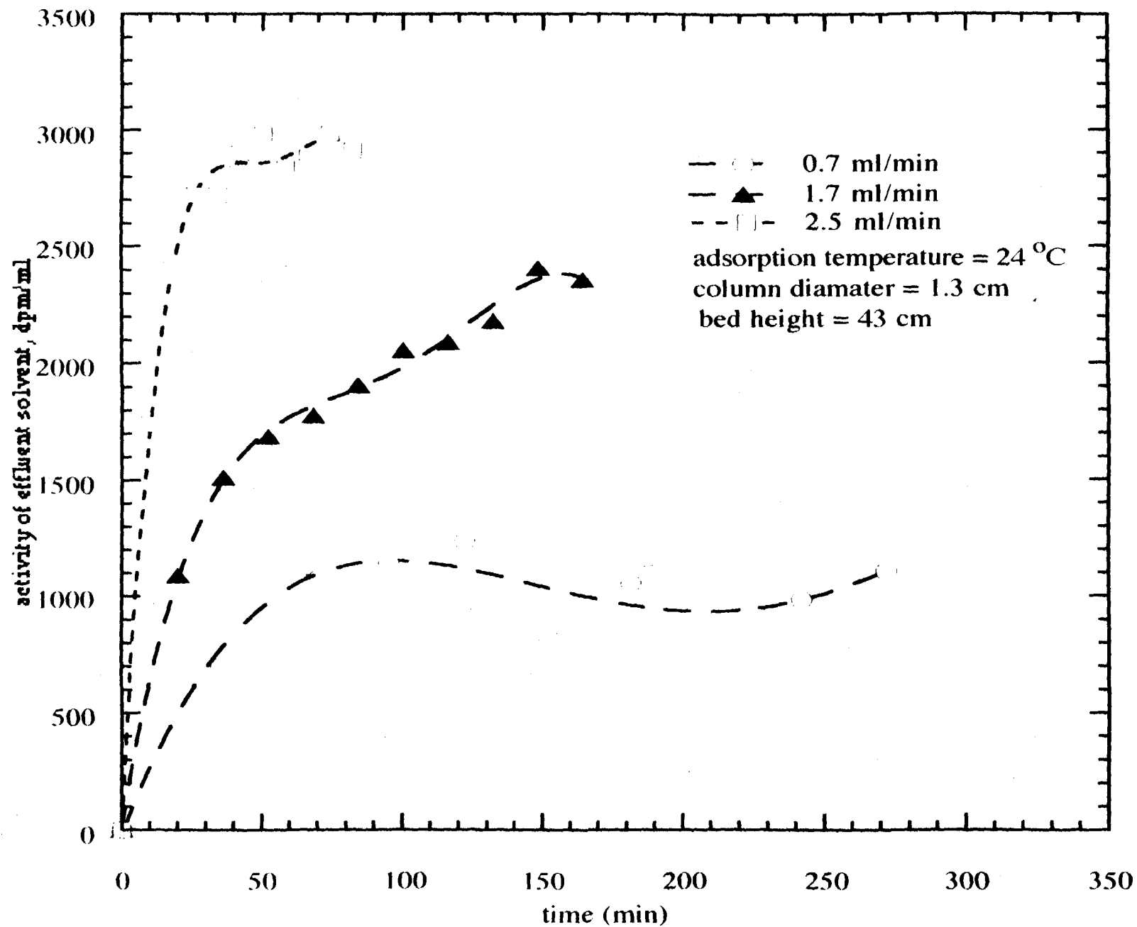
Figure 7. The effects of flow rate on adsorption of degradation products by activated alumina.
