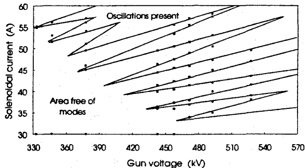
Fig. 6. Area of klystron self-oscillation at 3 \mu\text{s} operation. Coil current of 45 amps corresponds to an 1800 gauss axial field.
