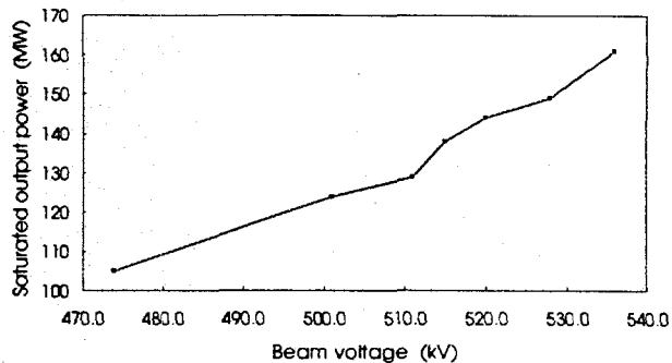
Fig. 8. Measured saturated output power ( 3 \mu\text{s} rf, 60 Hz). Severe changes in slope are due to gain variation with magnetic field.
