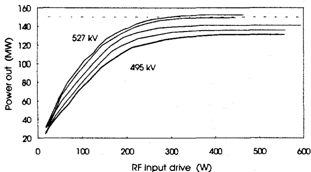
Fig. 7. Measured output power versus drive for the 150-MW klystron for 527, 523, 511, 503 and 495 kV. ( \mu\text{K}=1.8 , B_z=1800 \text{ g} , \tau=3 \mu\text{s} , Rep rate=60 Hz)
