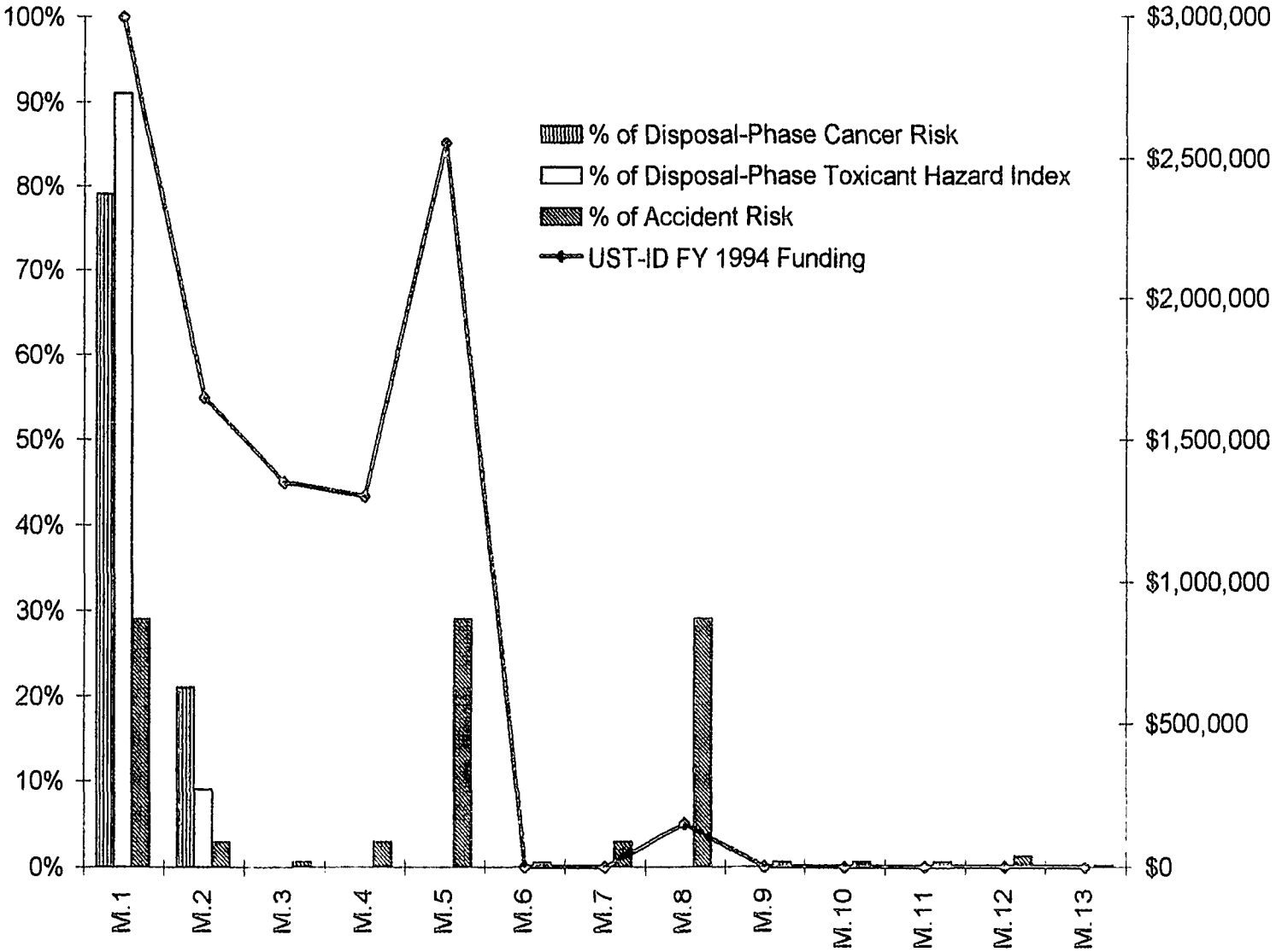
Figure 7. Comparison of UST-ID FY 1994 Funding to Selected Risks Evaluated for Thirteen Base Case Modules.
