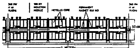
Fig. 1 2-m module in the main TBA.
