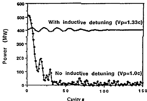
Fig. 2 Power extraction from 150-cavities in one unit of RK-TBA.
