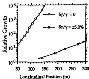
Fig. 4 Low frequency BBU growth, with and without Landau damping.
