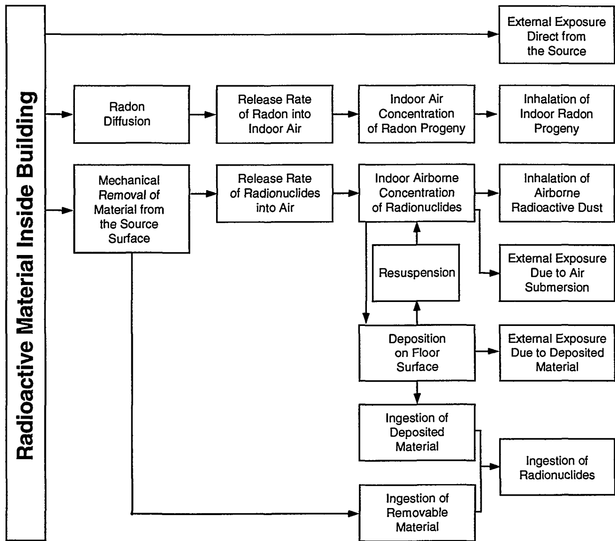
FIGURE 2. Schematic Representation of RESRAD-BUILD Pathways (Source: Yu 1994)
