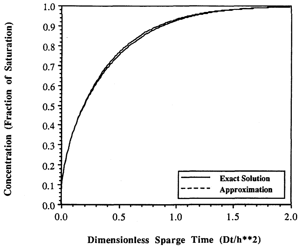
Figure 13. Comparison of Bulk Mass Transfer Approximation with Exact Solution of Diffusion Equation
