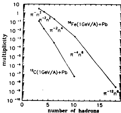
Fig.3. Multiplicities of exotic clusters as a function of the hadron number in the cluster for the collisions of ^{12}\text{C} and ^{56}\text{Fe} projectiles with the ^{208}\text{Pb} -target at 1 GeV/nucleon.
