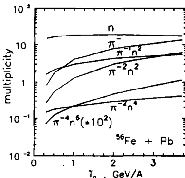
Fig.2. The same as in Fig.1, but for the ^{56}\text{Fe} -projectile.
