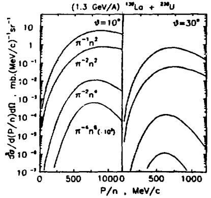
Fig. 7. Differential cross sections for pineut production in ^{139}\text{La} + ^{238}\text{U} collisions at 1.3 GeV/nucleon.
