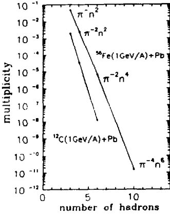
Fig. 6. Pineut yields calculated with the coalescence radius of 100 MeV/c.
