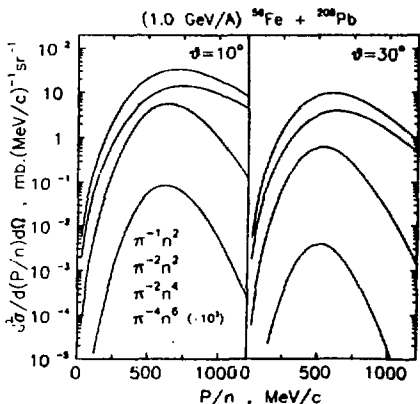
Fig.5. The same as in Fig.4, but for the ^{56}\text{Fe} projectile at 1 GeV/nucleon.
