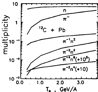
Fig.1. Multiplicity of pineuts produced in the lead target by ^{12}\text{C} with the energy in the range (0.3–3.7) GeV/A. Calculations were made in the framework of the coalescence model with p_0 = 200 MeV/c. Multiplicities of pions and neutrons were obtained by the firestreak model.
