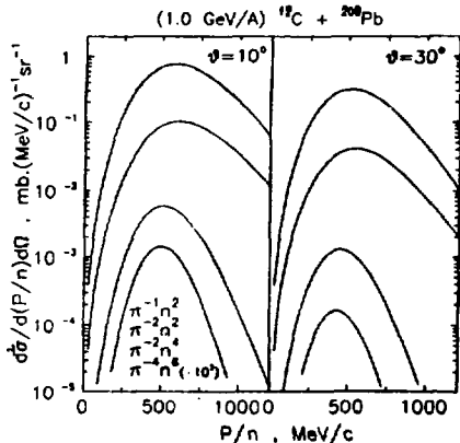
Fig.4. Differential cross sections for production of \pi^- n^2 , \pi^- n^2 , \pi^- n^4 , \pi^- n^6 in ^{12}\text{C} and ^{208}\text{Pb} collisions at 1 GeV/nucleon. Cross sections for \pi^- n^6 are shown with the factor of 10^3 . The same is valid for Figs.5 and 7, too.
