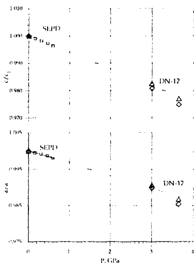
Fig.5. Dependences of the Hg-1212 lattice parameters on pressure, normalized to the values at P=0 . Points obtained on DN-12 and SEP are shown. Lines are drawn by the least square method. The lines drawn for c through both sets of data are indistinguishable.
