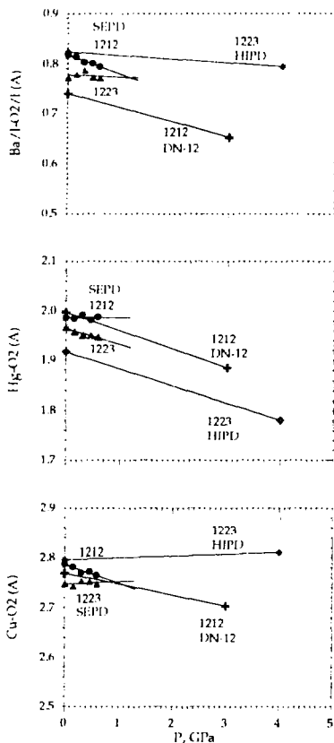
Fig.6. Interatomic distances in Hg-1212 and Hg-1223 as determined from the measurements on DN-12, SEPD, and HHPD. The lines are drawn by the least square method.
