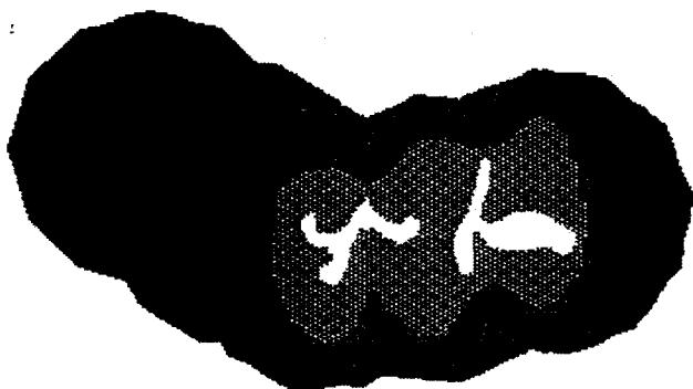
Figure 1: Schematic of the Carbon Black Aggregate Structure: A representative structure derived from SANS and high resolution microscopy of a typical HSA carbon black aggregate. 3 The structure consists of a linear array of spheroid particles. The average aggregation number is 4 to 6 with particle sizes being in the range of 240 to 290 Å. The outer shell of the structure (black) consists of graphitic carbon crystallites, with a core (gray) of less dense void-filled (white) carbon. The less dense core is contiguous throughout the aggregate.
