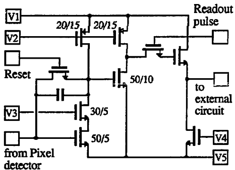
Fig. 10 Polysilicon TFT charge sensitive amplifier
