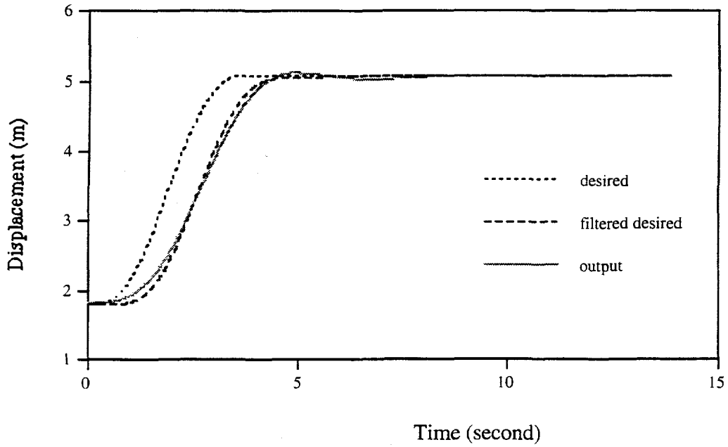
Fig. 4. Experimental results of the feedforward simulation filtering method.
