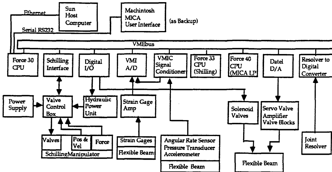
Fig. 2. VME system controller for the flexible-beam test bed.
