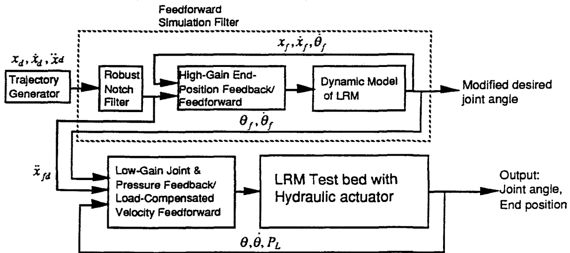
Fig. 3. The feedforward simulation filtering method.
