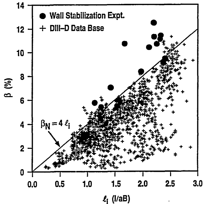
Fig. 6. The DIII-D high \beta database indicates that the best achievable \beta increases approximately linearly with \ell_i , \beta_{max} \approx 4\ell_i I/aB . Recent experiments using wall stabilization (shown as solid dot) have been able to exceed this level.
