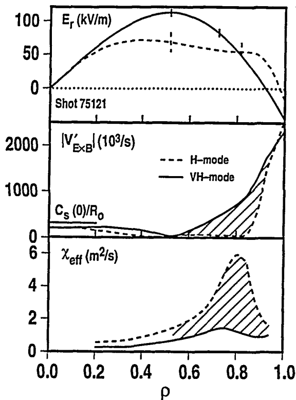
Fig. 3. Profile comparisons between H-mode (dashed lines) and VH-mode (solid lines). After the H-VH transition, in the region 0.6 \leq \rho \leq 0.9 , the V_{E \times B} shear increases and the effective thermal diffusivity is reduced.
