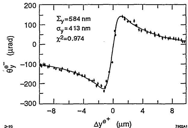
Fig 4. Beam-beam deflection, \theta , vs. separation, \Delta y , fitted with Bassetti-Erskine formula showing 413 nm vertical rms beam size.
