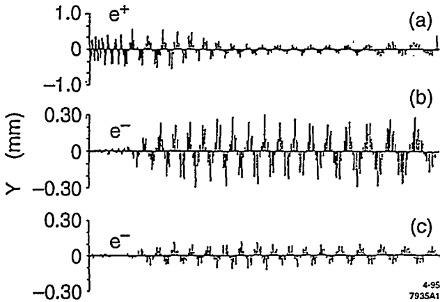
Fig 3. Vertical e^+ oscillation introduced before the linac (a) and long range wakefield induced oscillation for e^- beam of \sim 300 \mu\text{m} before (b) and \sim 100 \mu\text{m} after (c) installation of split tune lattice.
