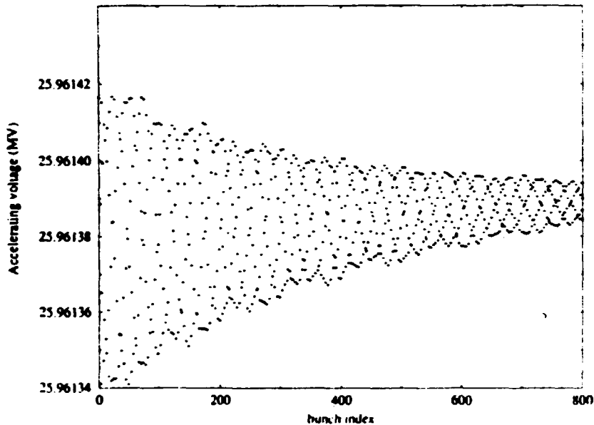
Figure 4 : Accelerating voltage evolution during 800 bunches
