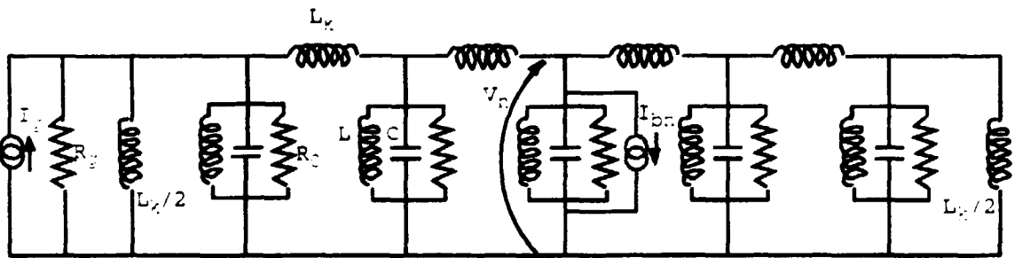
Figure A-2 : Equivalent circuit (with lumped elements in parallel)
