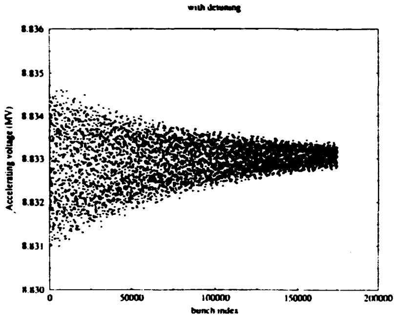
Figure 10 : Energy gain evolution on a longer time-scale (with cavity detuning).
