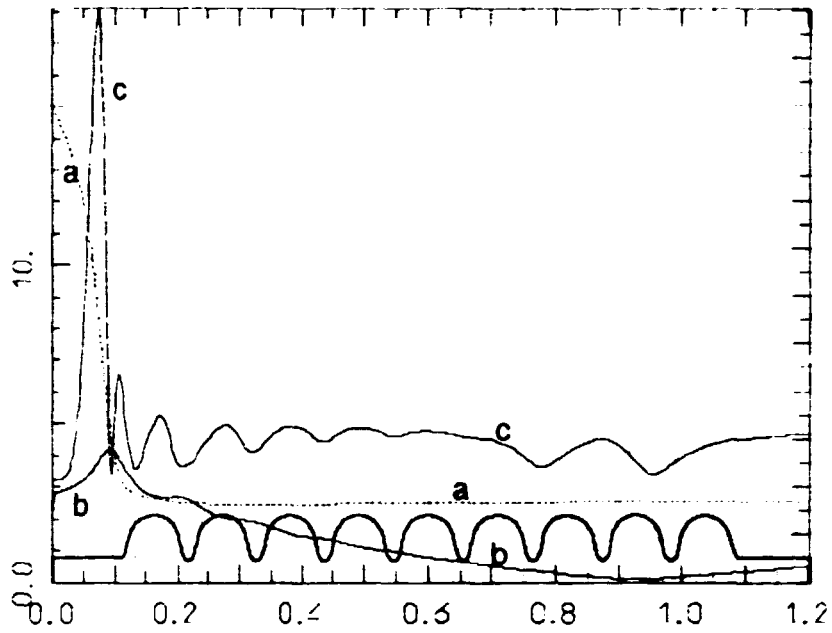
Figure 11: Single bunch computation: a-Bunch length [mm], b-Bunch radius [mm], c-rms norm. transv. emittance [mm mrad], versus z [m]
