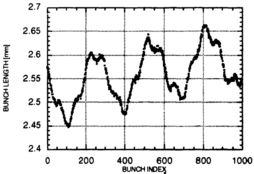
Figure 12: Bunch Length [mm]
