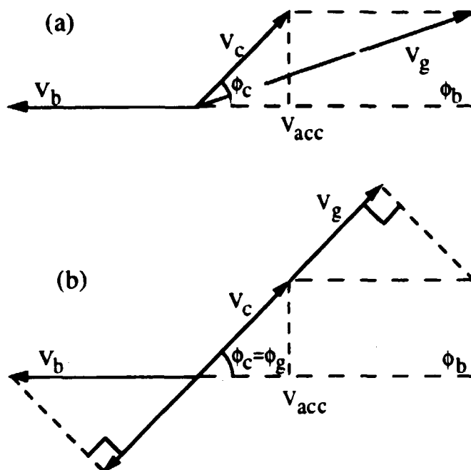
Figure 6 : Phasors diagram without (a) and with cavity detuning (b)
