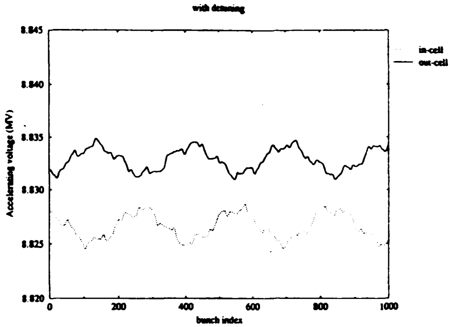
Figure 8 : Energy gain evolution with cavity detuning.
