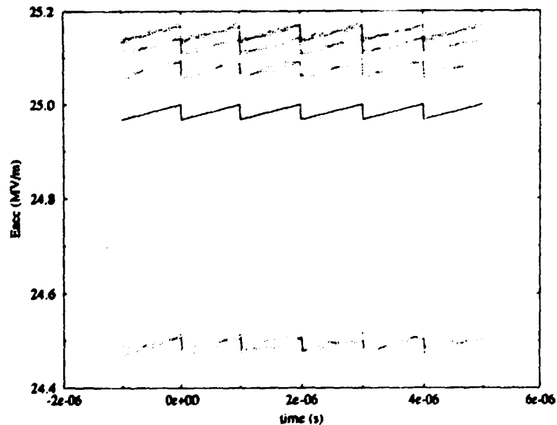
Figure 3 : cell accelerating fields and average with a relativistic bunch train
