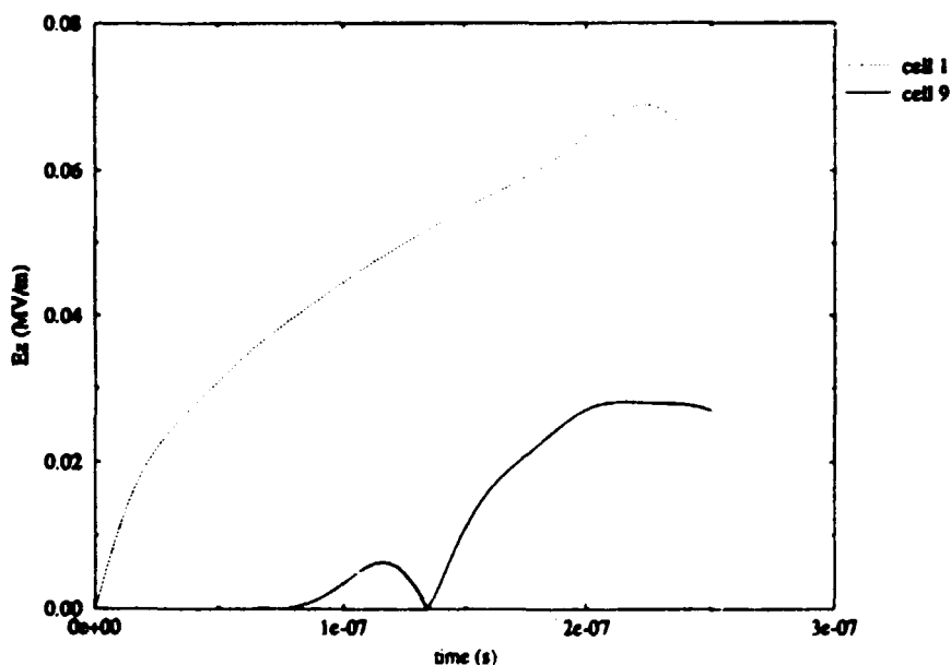
Figure 1 : field envelope at center of cells during the cavity filling
