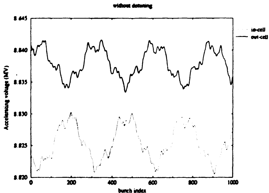
Figure 7 : Energy gain evolution without cavity detuning
