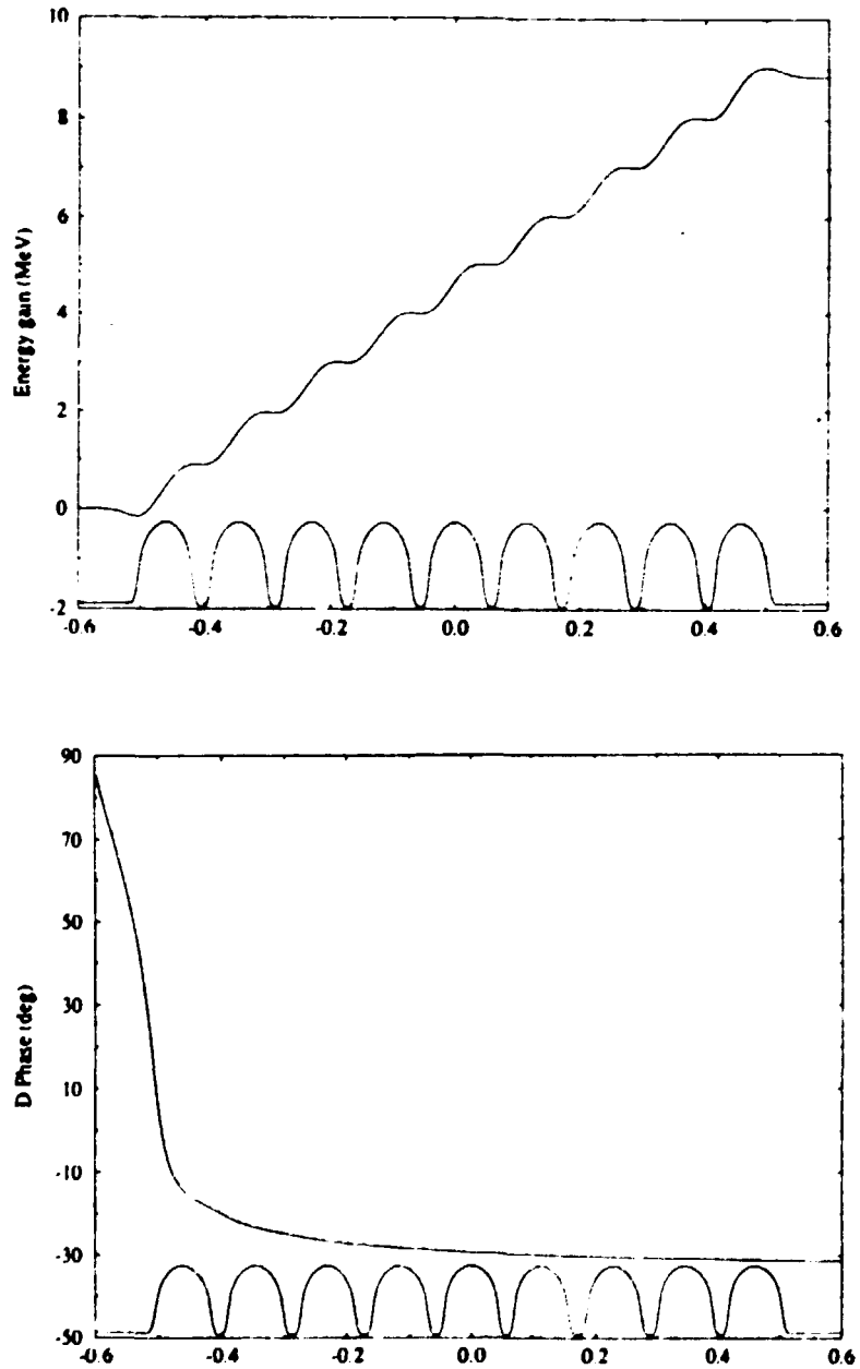
Figure 5 : Energy gain and beam phase shift along the SC capture cavity (the cavity profile is also shown)
