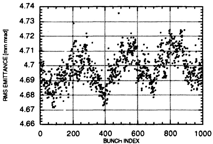
Figure 14: Rms Normalized Emittance [mm mrad]
