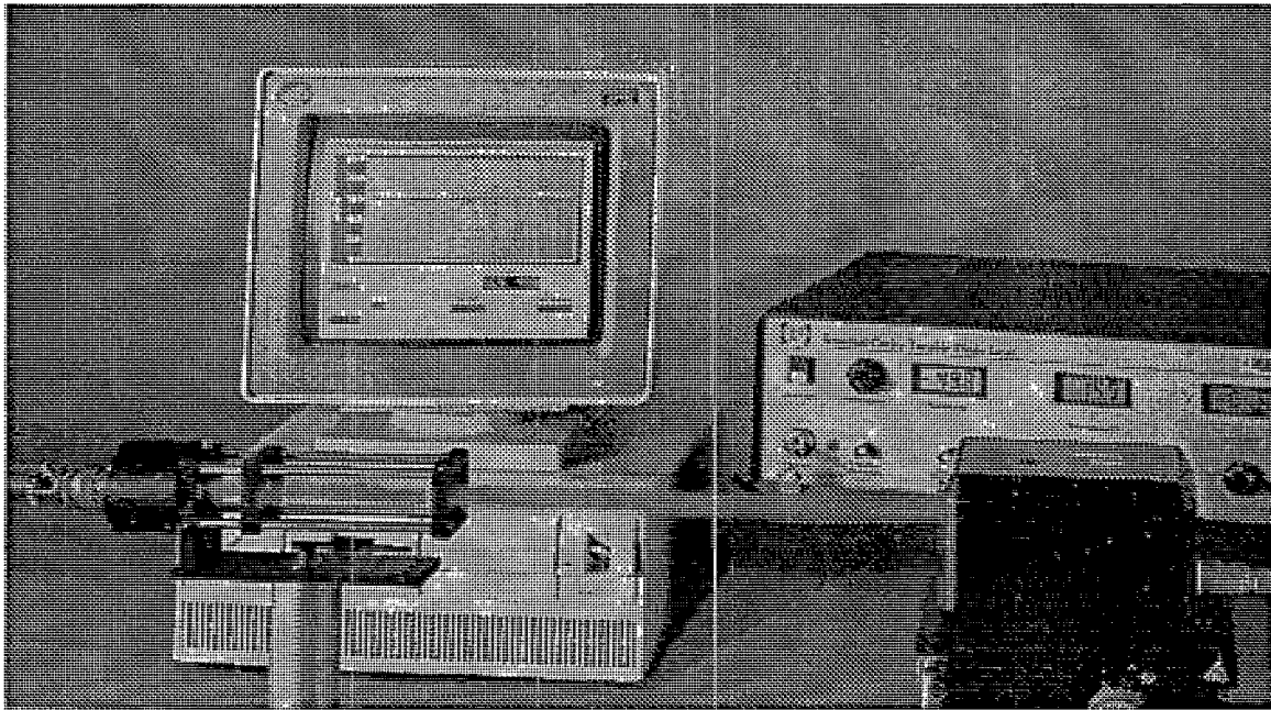
Figure 3 - Prototype of diode laser based vapor monitor.
