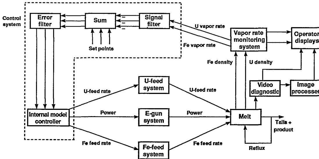
Figure 6 - Models based, closed loop vaporizer control system.
