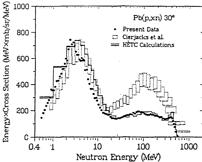
Figure 1: Comparison of neutron production cross-sections (multiplied by the energy) for 585 and 597 MeV protons on lead obtained by two different groups. From Ref.[2].
