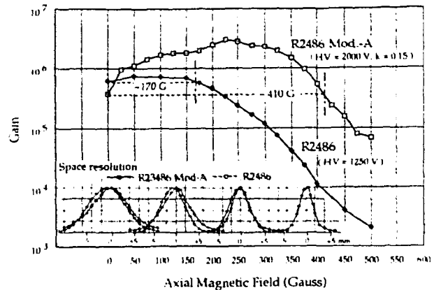
Figure 7. Comparison of Proto #2 to R2486.
