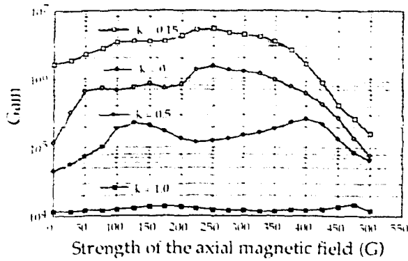
Figure 4. Gain variation of Proto #2 as a function of axial magnetic field.
