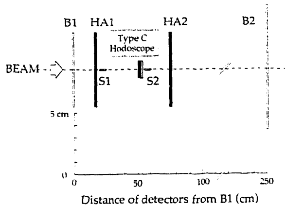
Figure 19. Experimental layout on T7-S.
