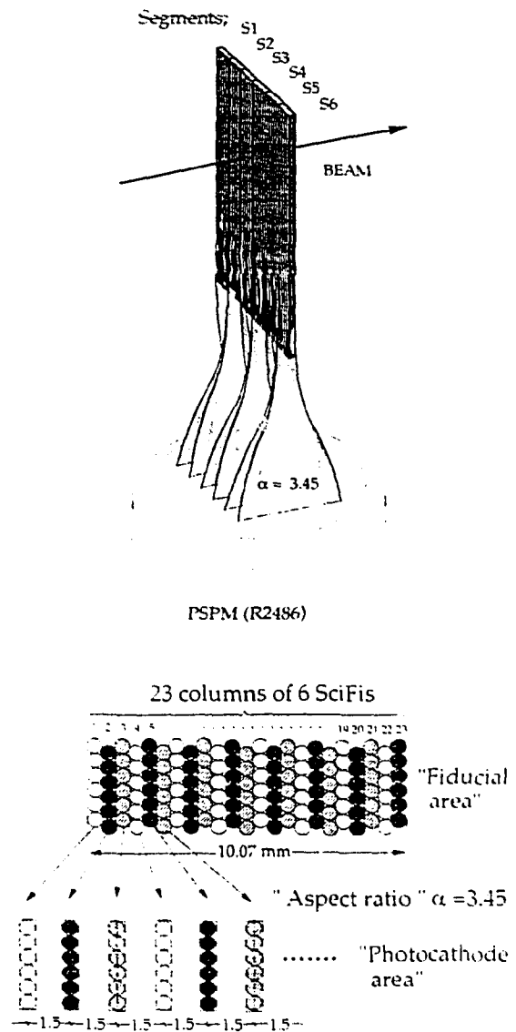
Figure 8. Mechanical structure of type A hodoscopes.
