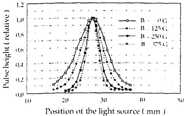
Figure 5. Secondary electron spread at different magnetic field.
