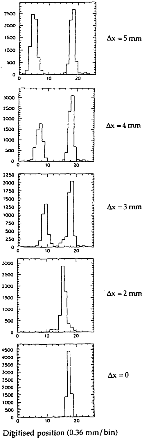
Figure 15. Real-time reconstruction of two-hit events using delay-line digitiser.
