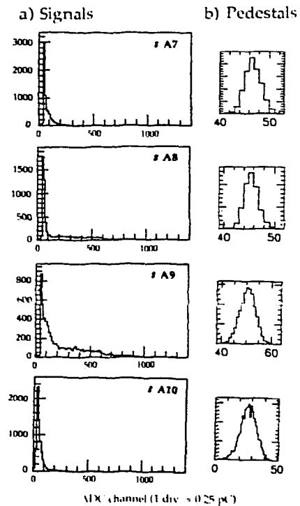
Figure 21. "Raw" spectra from adjacent anodes.
