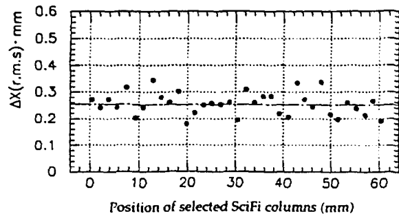
Figure 11. Spatial resolution at different positions.
