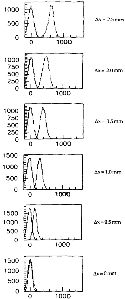
Figure 16. Reconstruction of two-hit events using "double-side" CFD.
