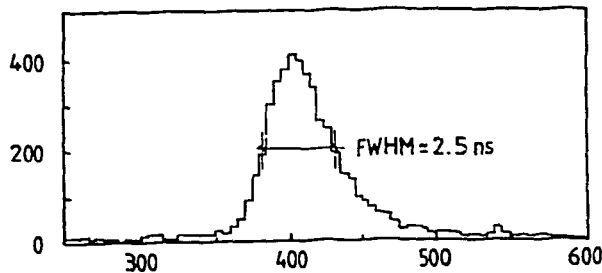
Figure 17. Mean-time, (t_1 + t_2)/2 , distribution with respect to the reference time t_0 defined by an external counter.
