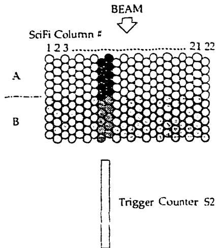
Figure 20. Double SciFi-arrays for "proximity" tracking.
