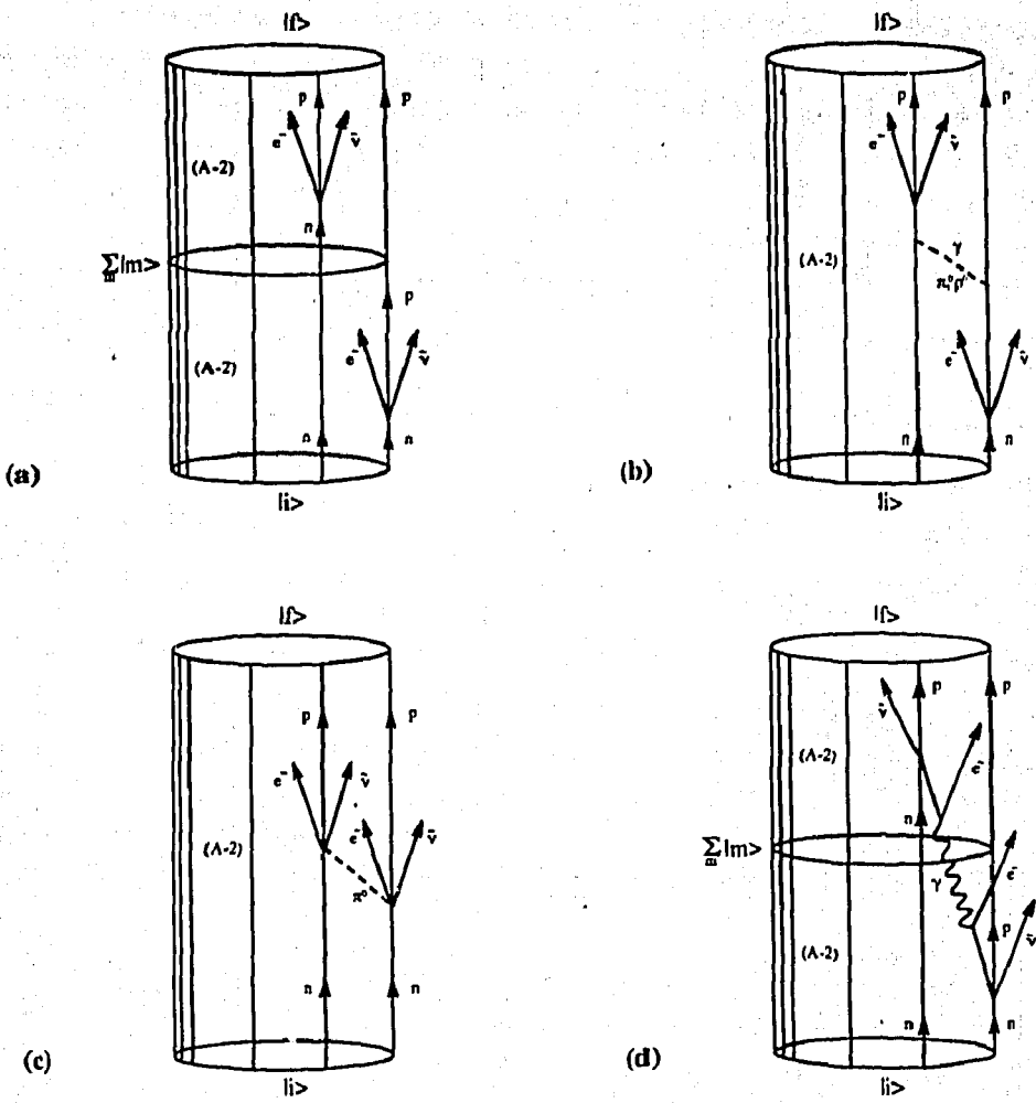
Figure 1: The Feynmann diagrams for the two subsequent nuclear beta decay processes and for the two neutrino nuclear double beta decay process. (a) The Feynmann diagram for two subsequent nuclear beta decays within the impulse approximation. (b) The Feynmann diagrams of the two neutrino double beta decay process of the two nucleon mechanism considered at present. (c) The pion exchange mechanism of the two neutrino double beta decay process of Ericson and Vergados. (d) The electron-gamma exchange mechanism of the two neutrino double beta decay process.
