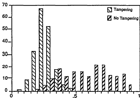
Fig. 3 - Histogram of pairwise spectra comparisons. These data were obtained in an operating vault under variable conditions. Separation of tamper from no-tamper cases is much worse than in the controlled laboratory setting (Fig. 3), suggesting some operational limitation of the intrinsic seals technique.
