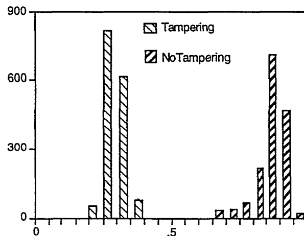
Fig. 3 - Histogram of pairwise spectra comparisons. These data were obtained in a laboratory setting and show clean separation of cases where tampering occurred between measurements from cases where no tampering occurred between measurements.
