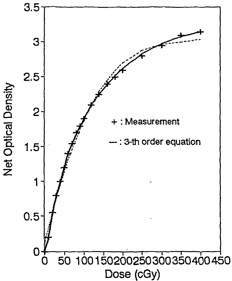
Fig. 3. H-D curve of Kodak X-Omat V film for Co-60.
