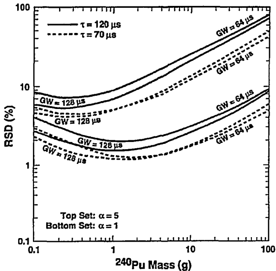
Fig. 3. Assay precision for passive neutron multiplicity assay of waste, for the case where the multiplicity information is used to solve for mass, multiplication, and (\alpha, n) reaction rate. Detector efficiency = 35% and background = 10 counts/s. The dependence of assay precision on gate width and die-away time is illustrated for \alpha = 1 and \alpha = 5 .
