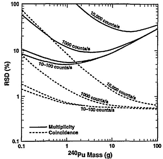
Fig. 8. Assay precision for passive neutron coincidence and multiplicity assay of waste, for the case where the multiplicity information is used to solve for mass, detector efficiency, and (\alpha, n) reaction rate. Detector efficiency = 35\% , gate width = 128 \mu\text{s} , die-away time = 120 \mu\text{s} , and \alpha = 1 . The dependence of assay precision on background is illustrated.
