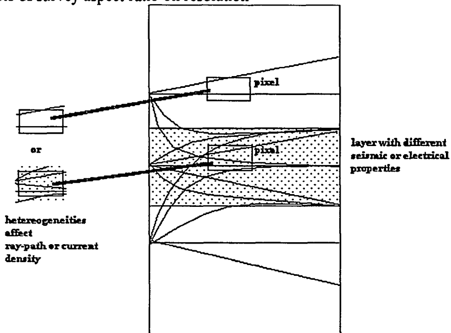
Figure 9b: Effects of subsurface heterogeneities on resolution
