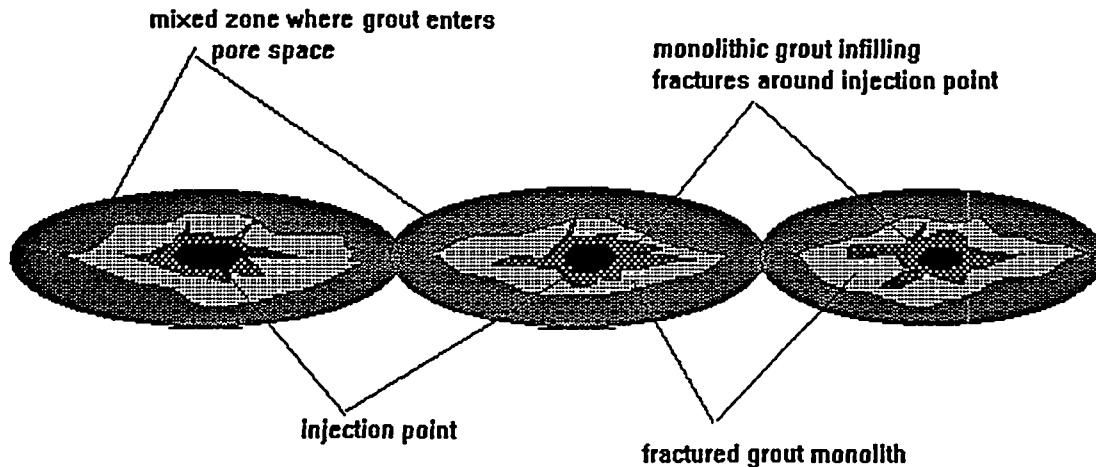
Figure 3: Conceptual Cross-Section of Subsurface Grout Barrier
