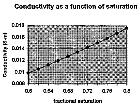
Figure 6: The relationship between soil saturation and electrical conductivity for a typical sandy soil of the Chemical Waste Landfill (assuming 30% porosity and a range of saturation from 0.6 to 0.8). A change in saturation from 0.7 to 0.6 would result in a reduction in conductivity from 0.013 to 0.010 S-m, which is on the order of the observed contrasts in the electromagnetic images of the site.
