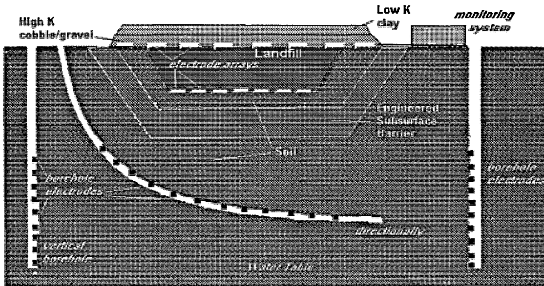
Figure 4: Possible configuration for electrical monitoring system
