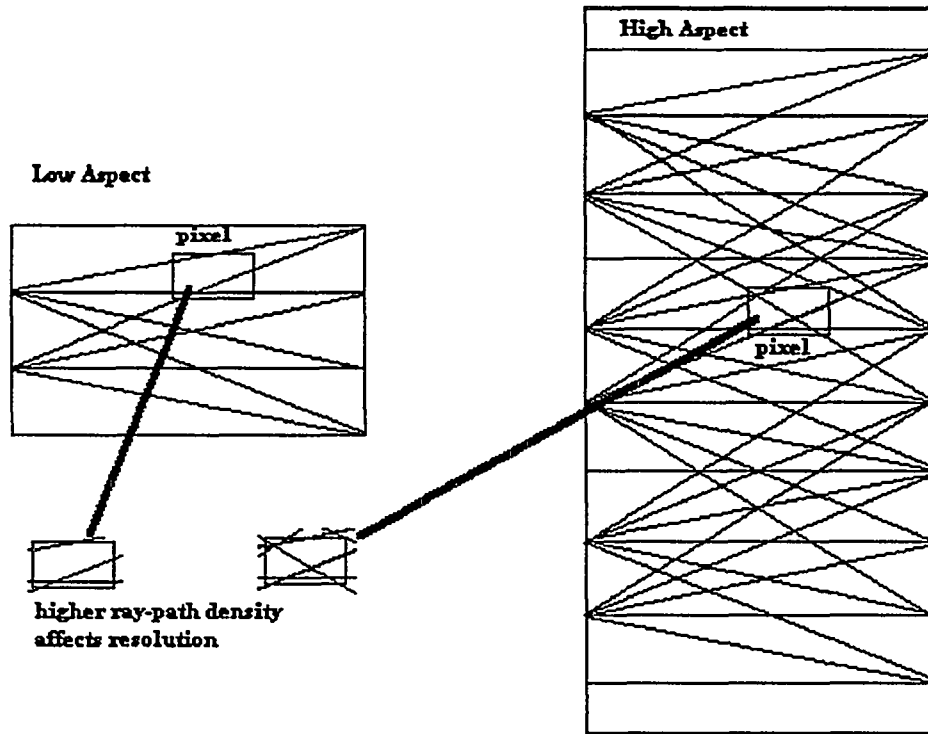
Figure 9a: Effects of survey aspect ratio on resolution
