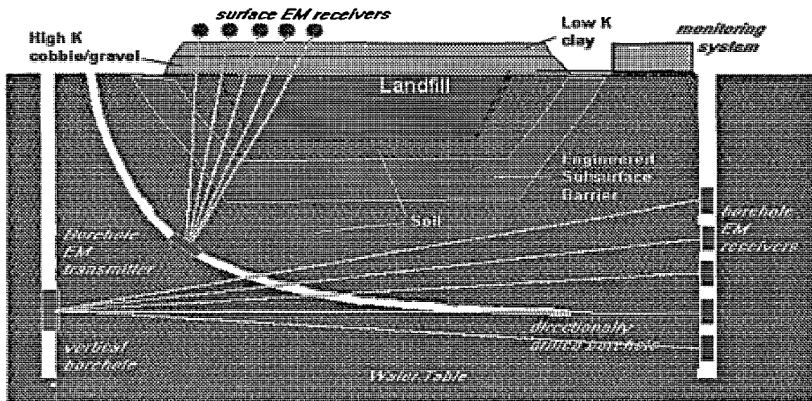
Figure 5: Possible configuration for electromagnetic or seismic system for monitoring or characterization
