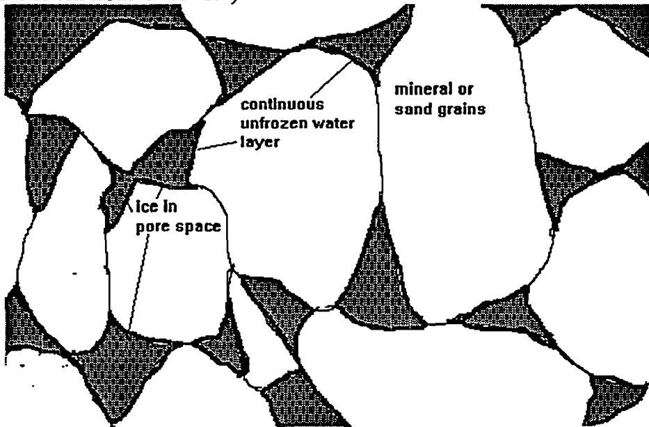
Figure 2. The structure of frozen soil, showing the continuous layer of adsorbed water on mineral grains (from King, et al., 1988)
