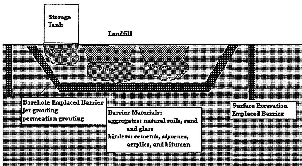
Figure 1: Conceptual Barrier Emplacement
