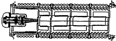
Figure 1: Schematic of the ESQ injector showing the diode column and the electrostatic quadrupoles.
