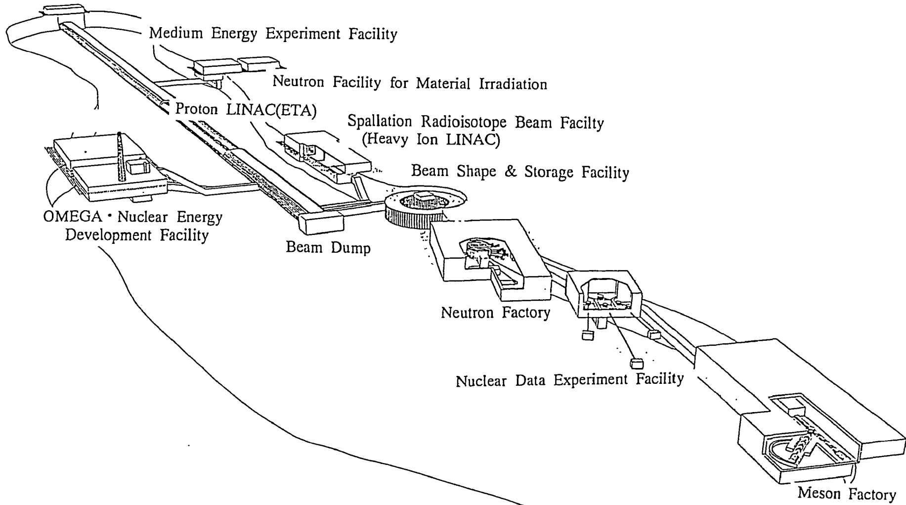
Fig.1 A Bird-Eye Figure of ETA and Research Facilities
