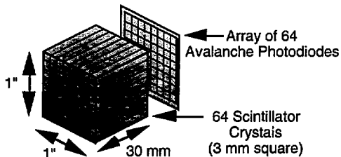
Fig. 8: Solid State Photodetector PET Detector Module.
