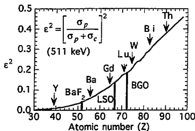
Fig. 5: Double Photoelectric Interaction Probability.
