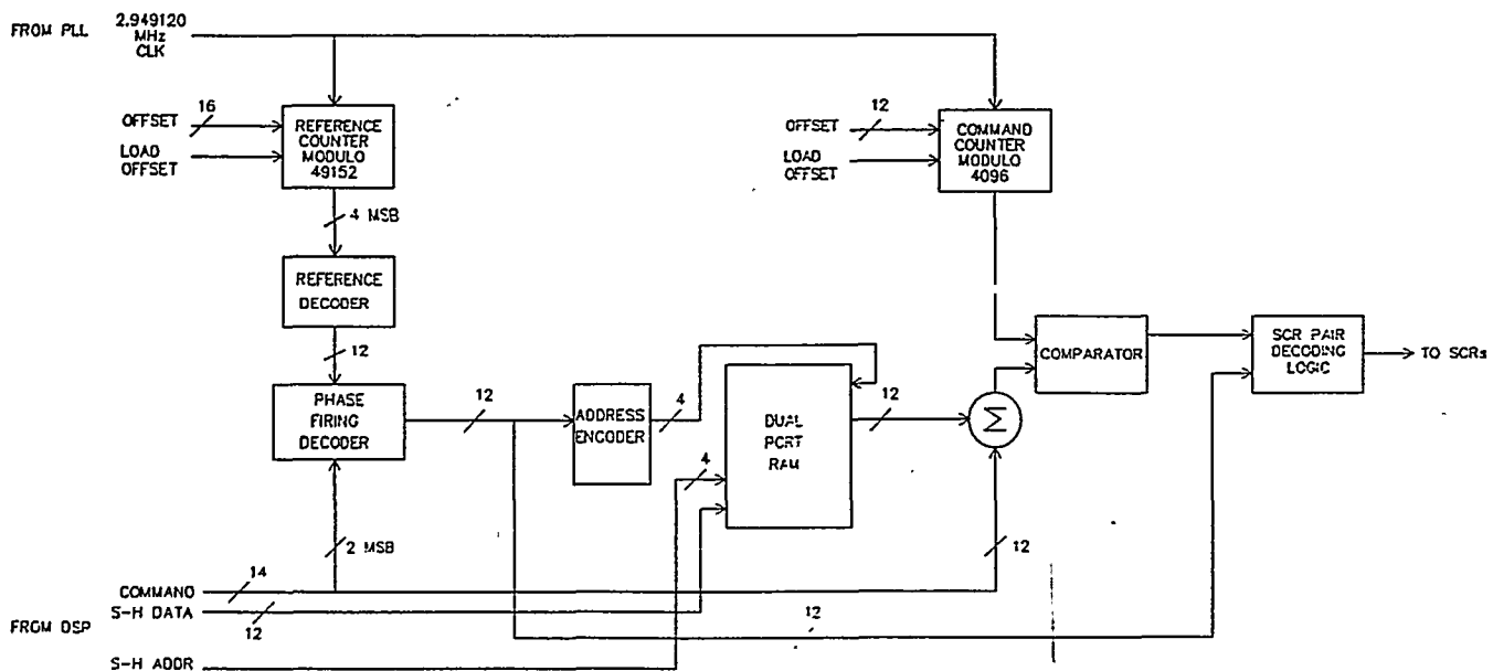
Figure 1 Digital Firing Circuit Block Diagram
