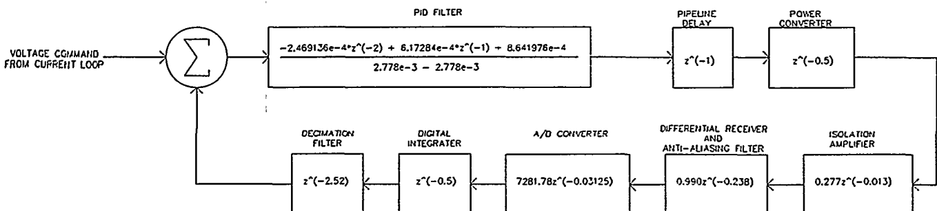
Figure 2 Voltage Loop Block Diagram
