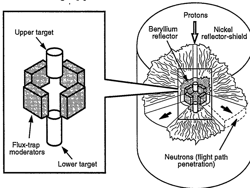
Figure 1. Illustration of the target system used at the MLNSC. The target system consists of a split target of tungsten, four flux-trap moderators of water and liquid hydrogen, an inner moderating reflector of beryllium, and an outer fast neutron reflector and high-energy neutron shield of nickel. The target system forms a right circular cylinder of about 1-m diameter and 1-m high.
