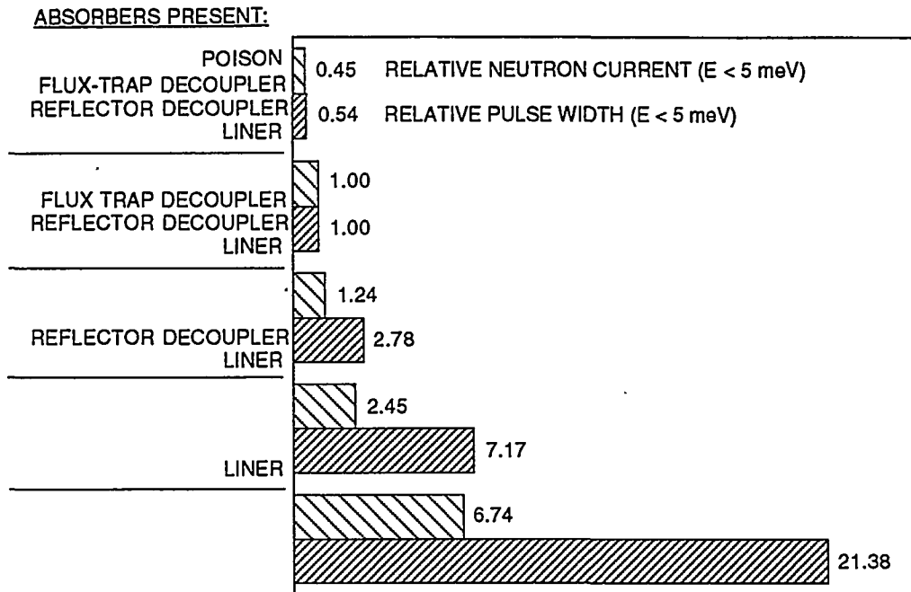
Figure 3. Effect of poisons, decouplers and liners on neutron pulse intensity and pulse width for liquid \text{H}_2 (ortho/para 50/50 v%) moderators. The labels on the left side of the bar graph indicate what items are present for the corresponding bars. The neutron pulse width is defined as the standard deviation of the time at which neutrons leak from the moderator viewed surfaces. The 22.5-cm-long, \text{D}_2\text{O} -cooled W rod-target is singly split and the four 5 \times 13 \times 13\text{-cm}^3 moderators are in flux-trap geometry. The poison is 0.00508-cm-thick Gd, and the decouplers and liners are 0.0813-cm-thick Cd. The reflector is \text{D}_2\text{O} -cooled Be ( \text{D}_2\text{O}/\text{Be} 15/85 v%). The proton beam energy is 800 MeV.
