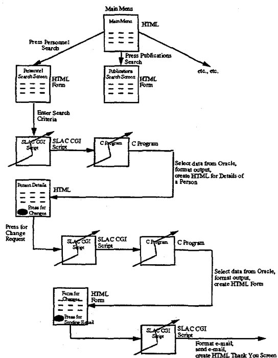
Fig. 7. Flow Chart of Web Database Queries to Send E-mail for Updating Personnel Information
