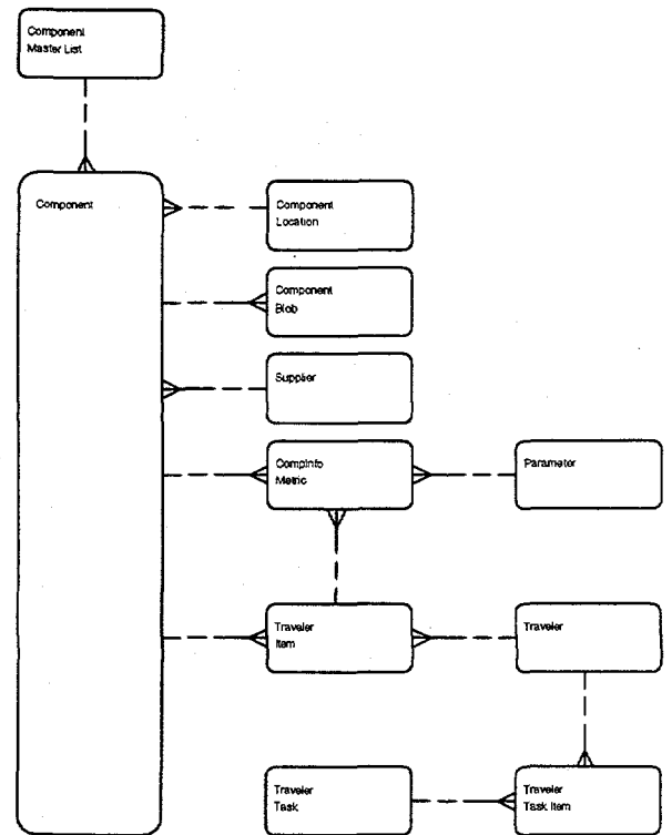
Fig. 3. Components, Travelers, Tasks and Metrics Entities and Relationships Diagram
