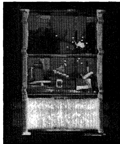
Figure 8 is a volume rendered image with fused SPECT reconstruction. The 133 Ba source is clearly visible as a white spot in the upper layer. A transparent bottle with free liquid laying on its side is also evident to the left of the 133 Ba source. Aerosol can and liquid level is rendered transparent in the center section of the phantom.
