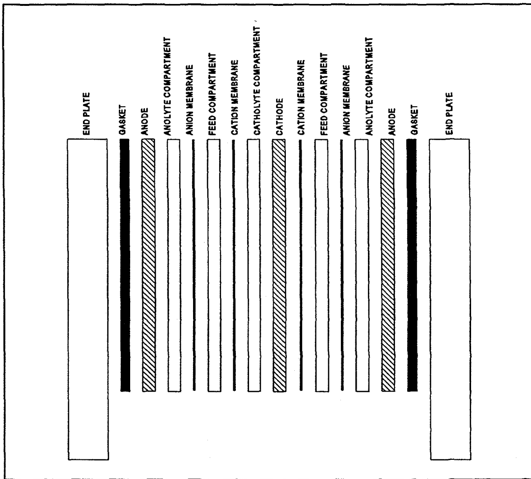
Figure 3. EDIX Cell Stack Configuration.
