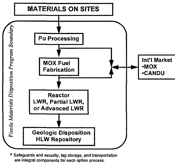
FIGURE 1. Reactor Alternatives
