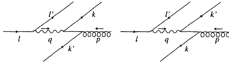
FIG. 1. Lowest order graphs contributing to the process: e + G^* \rightarrow l' + q + \bar{q} .
