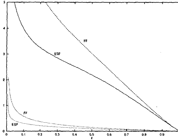
FIG. 3. Comparison of unpolarized d-quark distributions z f^{dB}(z) calculated by ESF and FF methods. The upper two lines result from contributions from all electroweak bosons while the lower two from \gamma\gamma only.
