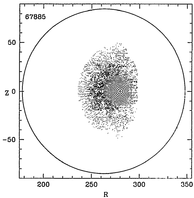
Fig. 16. Confinement domain in TFTR, equilibrium 67885.
