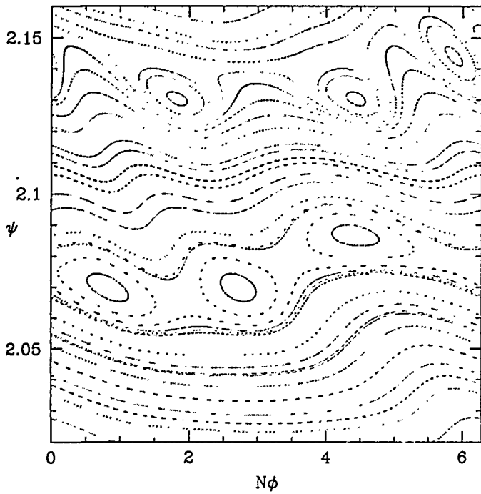
Fig. 10. Poincaré plot, \Delta = 0.01 , N\phi'_p = 1 , s_b = 0.05 .
