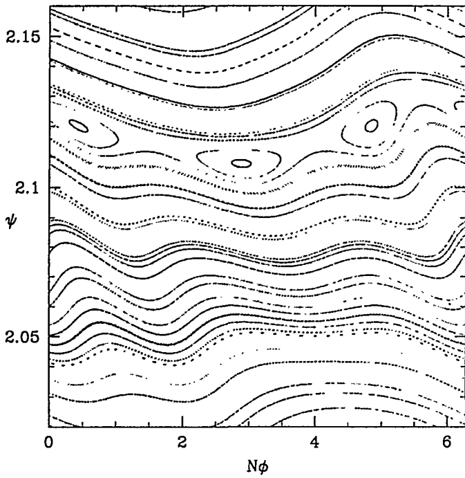
Fig. 8. Poincaré plot, \Delta = 0.01 , N\phi'_p = 1 , s_b = 0.08 .
