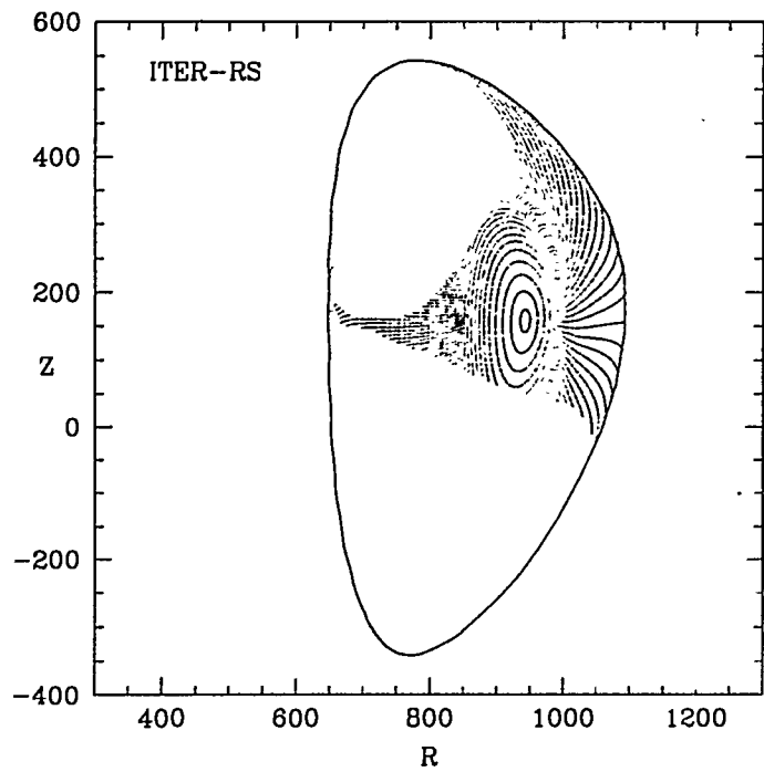
Fig. 18. Ripple well domain in ITER, reversed shear.
